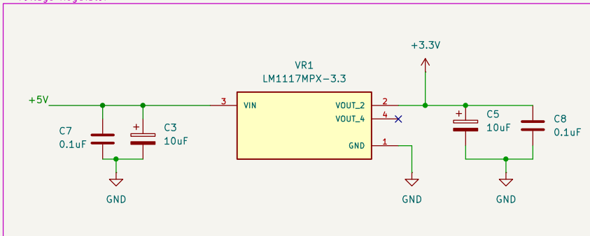
Voltage Regulator
