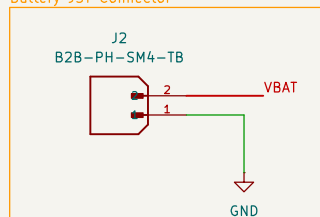
Battery JST Connector
