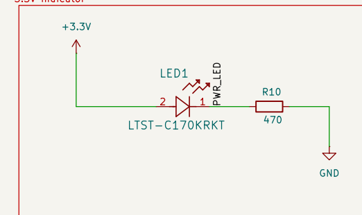
3.3V Indicator
