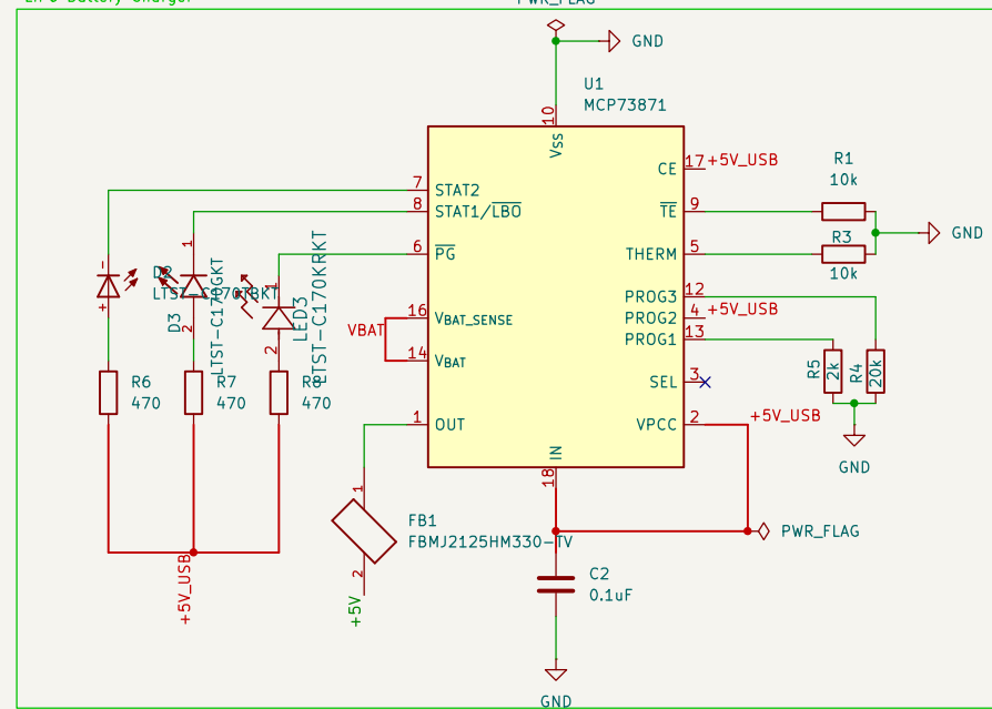
LiPo Battery Charger
