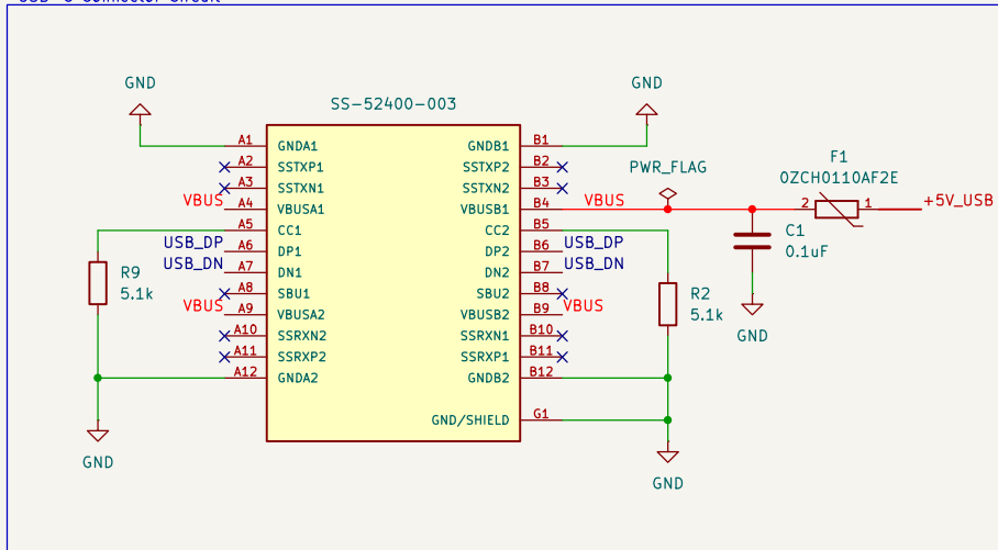
USB-C Connector Circuit
