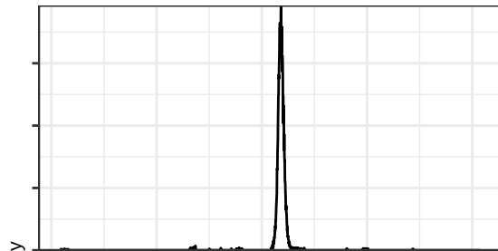
n-Methyl Glutamic Acid Standard
