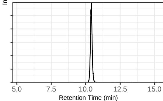
n-Methyl Glutamic Acid Standard
