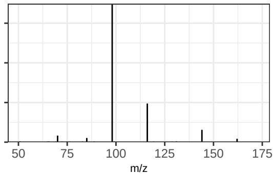
n-Methyl Glutamic Acid Standard
