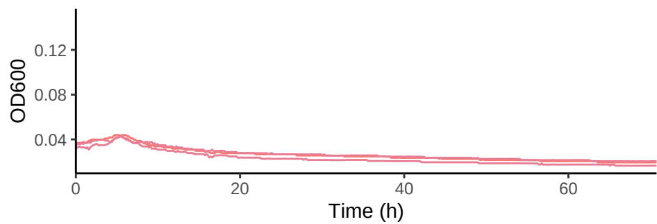
SPO3186_46D7 in Homarine 4 mM C with Kan 50
