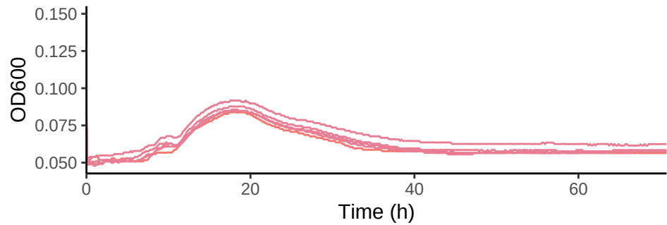
DSS3 in Glycine betaine 4 mM C with Kan 50
