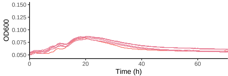
DSS3 (wt) in Glycine betaine 4 mM C
