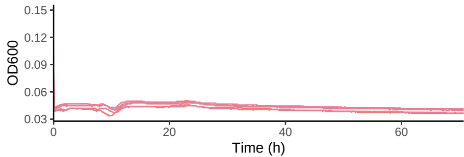
DSS3 (wt) in Carnitine 4 mM C
