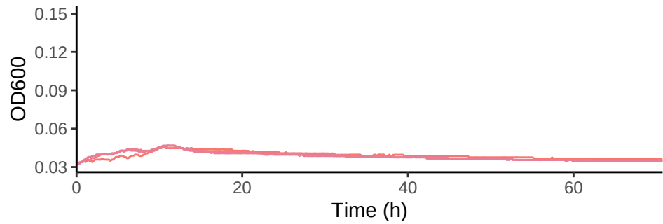
SPO3186_48115 in DMSP 4 mM C with Kan 50
