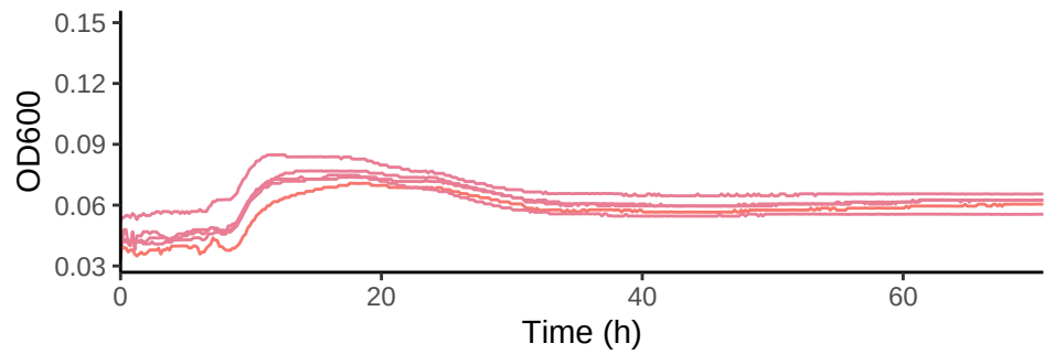
DSS3 in N-methyl-glutamic acid 4 mM C with Kan 50
