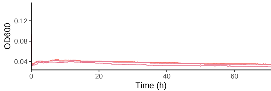
SPO3186_46D7 in DMSP 4 mM C with Kan 50
