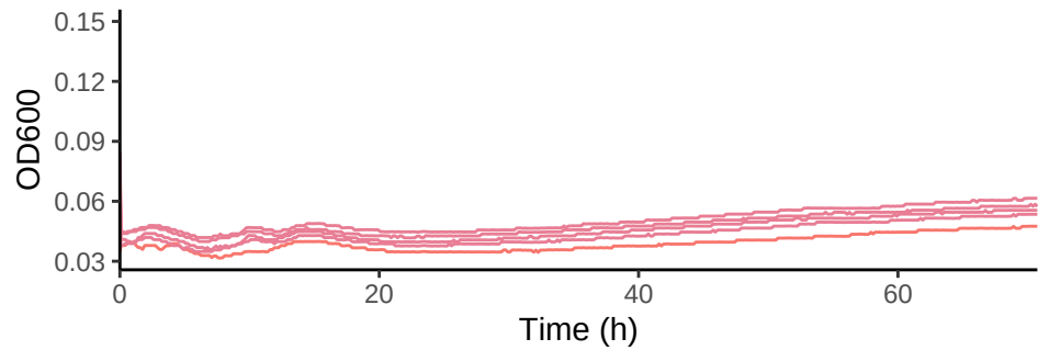
DSS3 (wt) in DMSP 4 mM C
