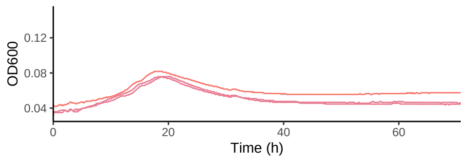
SPO3186_48115 in Homarine 4 mM C with Kan 50
