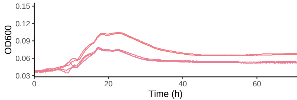
SPO3186_46D7 in N-methyl-glutamic acid 4 mM C wi
