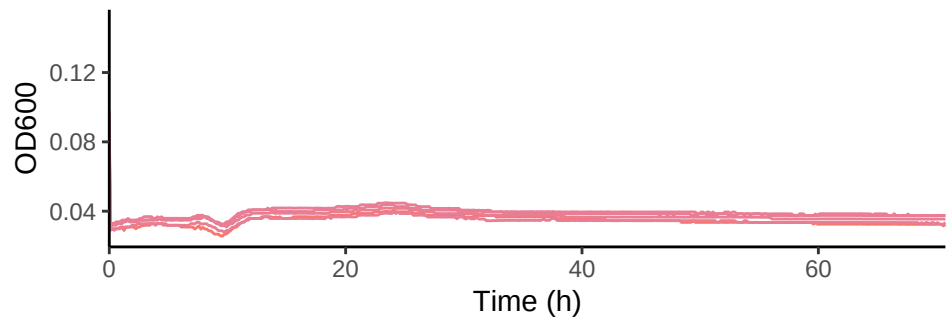
DSS3 in Carnitine 4 mM C with Kan 50
