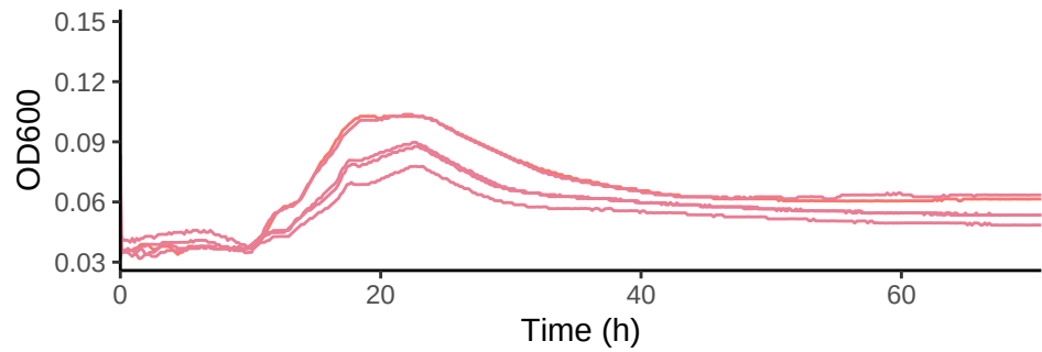
SPO3186_48115 in N-methyl-glutamic acid 4 mM C wi
