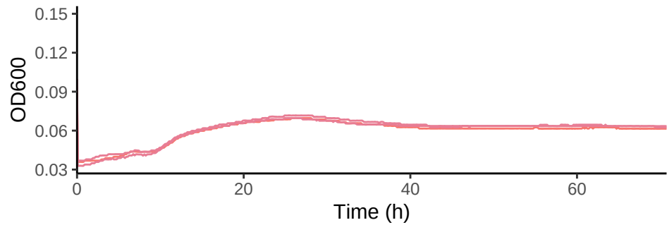
SPO3186_46D7 in Carnitine 4 mM C with Kan 50
