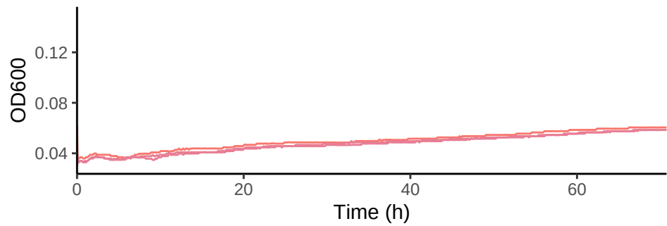
SPO3186_46D7 in Glycine betaine 4 mM C with Kan 50
