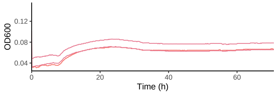
SPO3186_48115 in Carnitine 4 mM C with Kan 50
