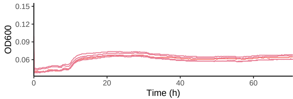
DSS3 (wt) in N-methyl-glutamic acid 4 mM C
