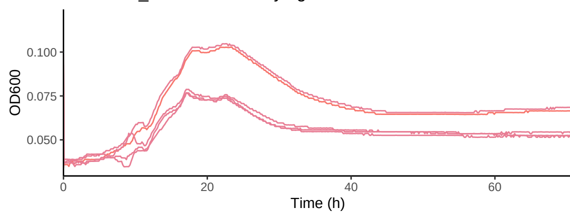
SPO3186_46D7 in N-methyl-glutamic acid 4 mM C with Kan 50
