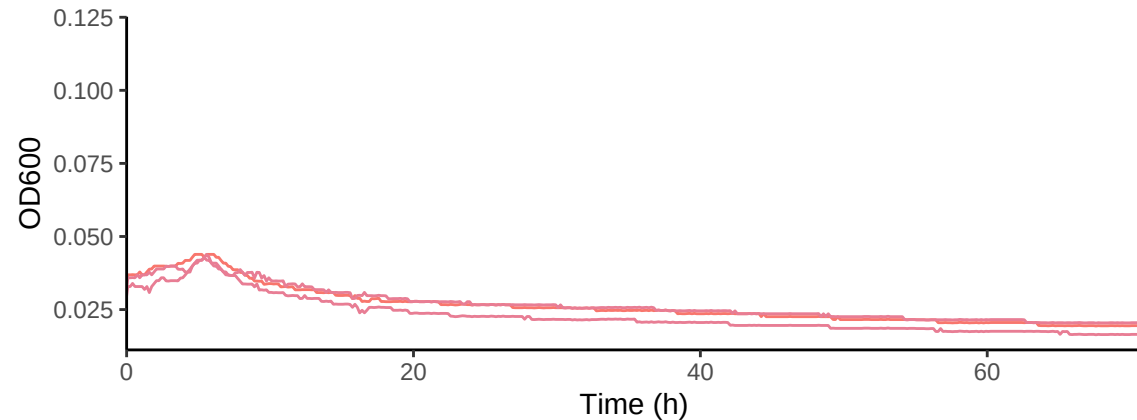
SPO3186_46D7 in Homarine 4 mM C with Kan 50
