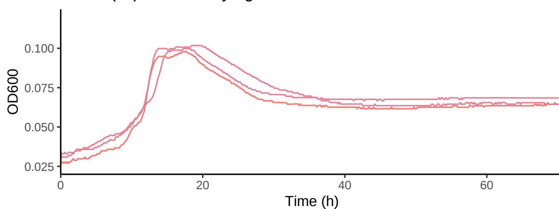
SPO3186_48115 in N-methyl-glutamic acid 4 mM C with Kan 50
