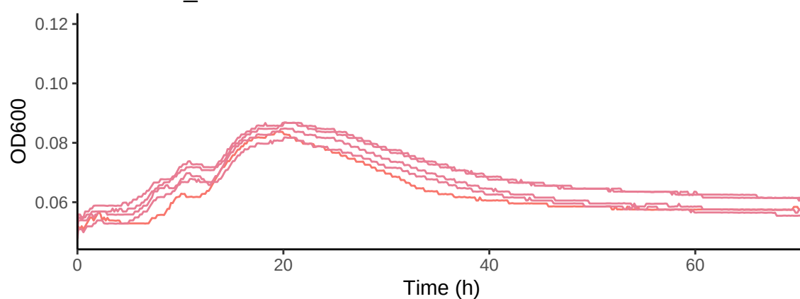
DSS3 (wt) in N-methyl-glutamic acid 4 mM C
