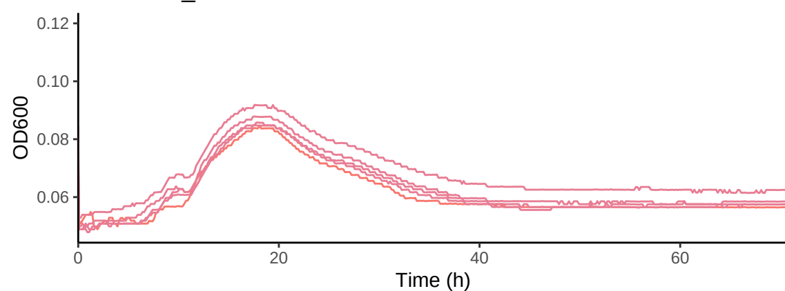
DSS3 in N-methyl-glutamic acid 4 mM C with Kan 50
