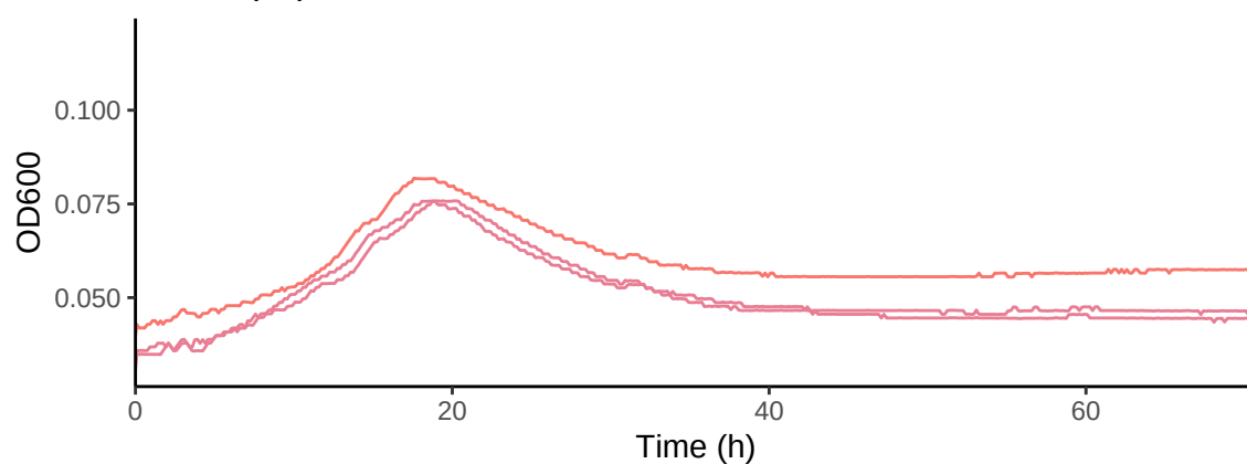
SPO3186_48115 in Homarine 4 mM C with Kan 50
