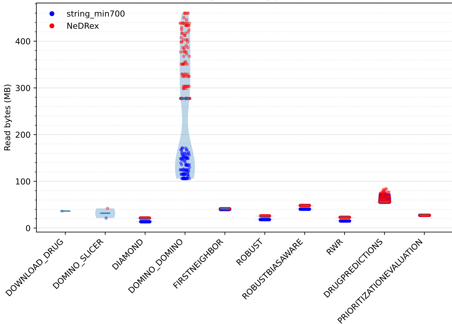
Read bytes (MB) by process
