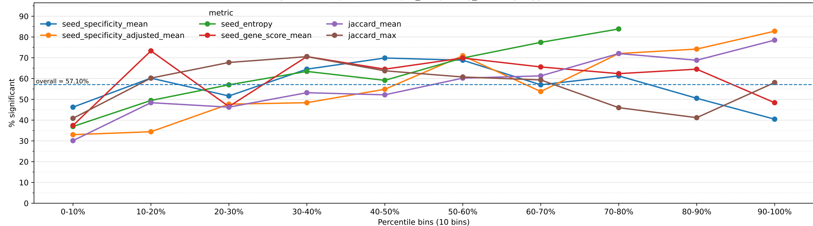
% significant vs quantile bins [per_sample, sig_rule=any, agg=median]
