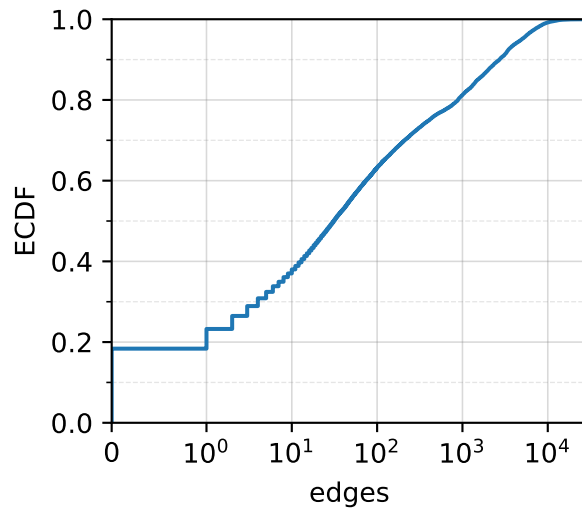
Empirical CDFs (unique per sample,ppi,algorithm)
