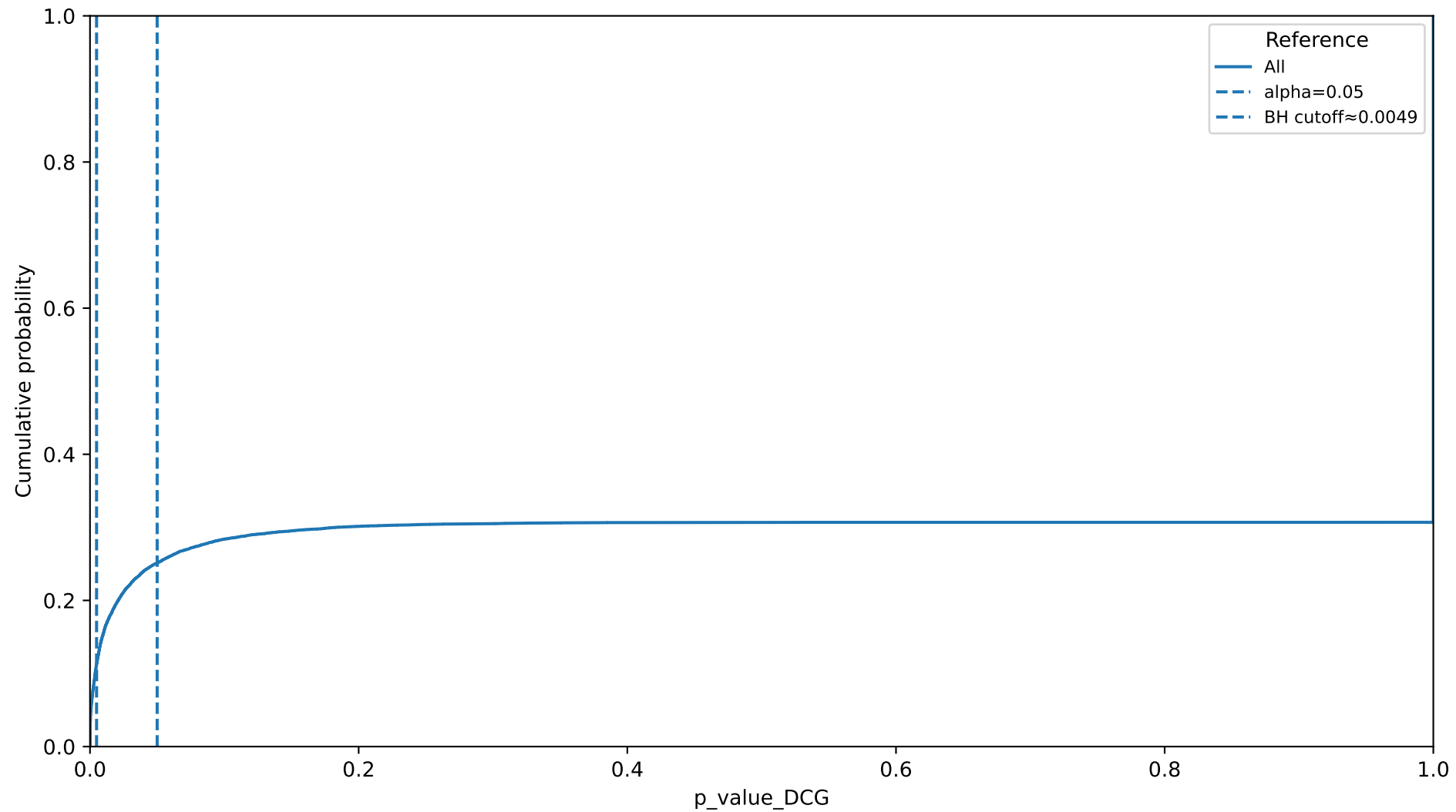
ECDF of DCG p-values (string_min700)
