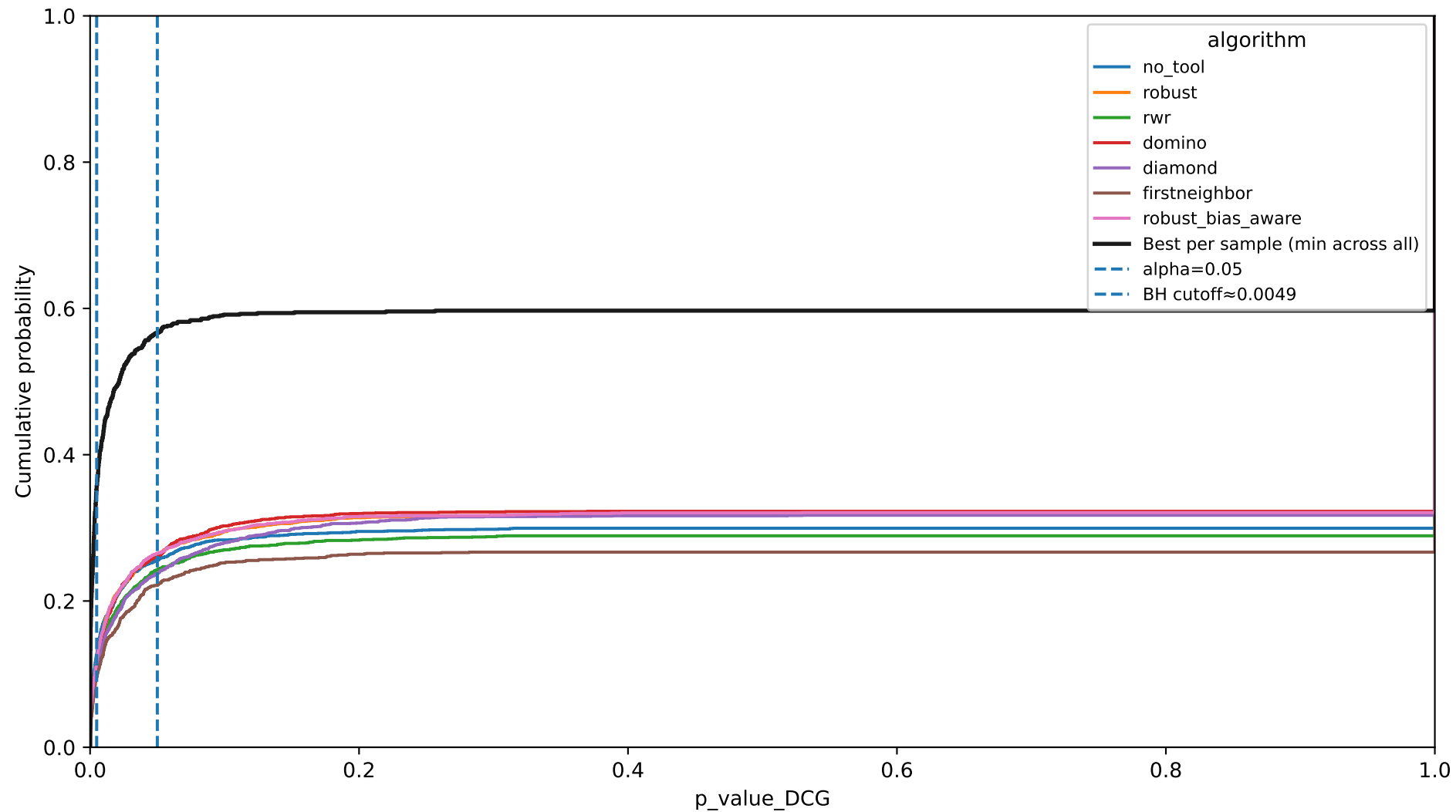
ECDF of DCG p-values by algorithm (string_min700)
