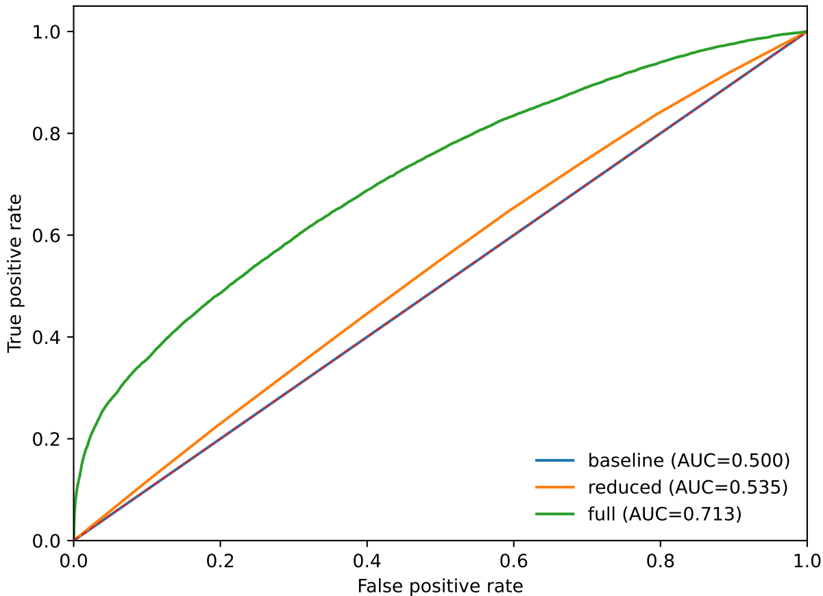
ROC curves
