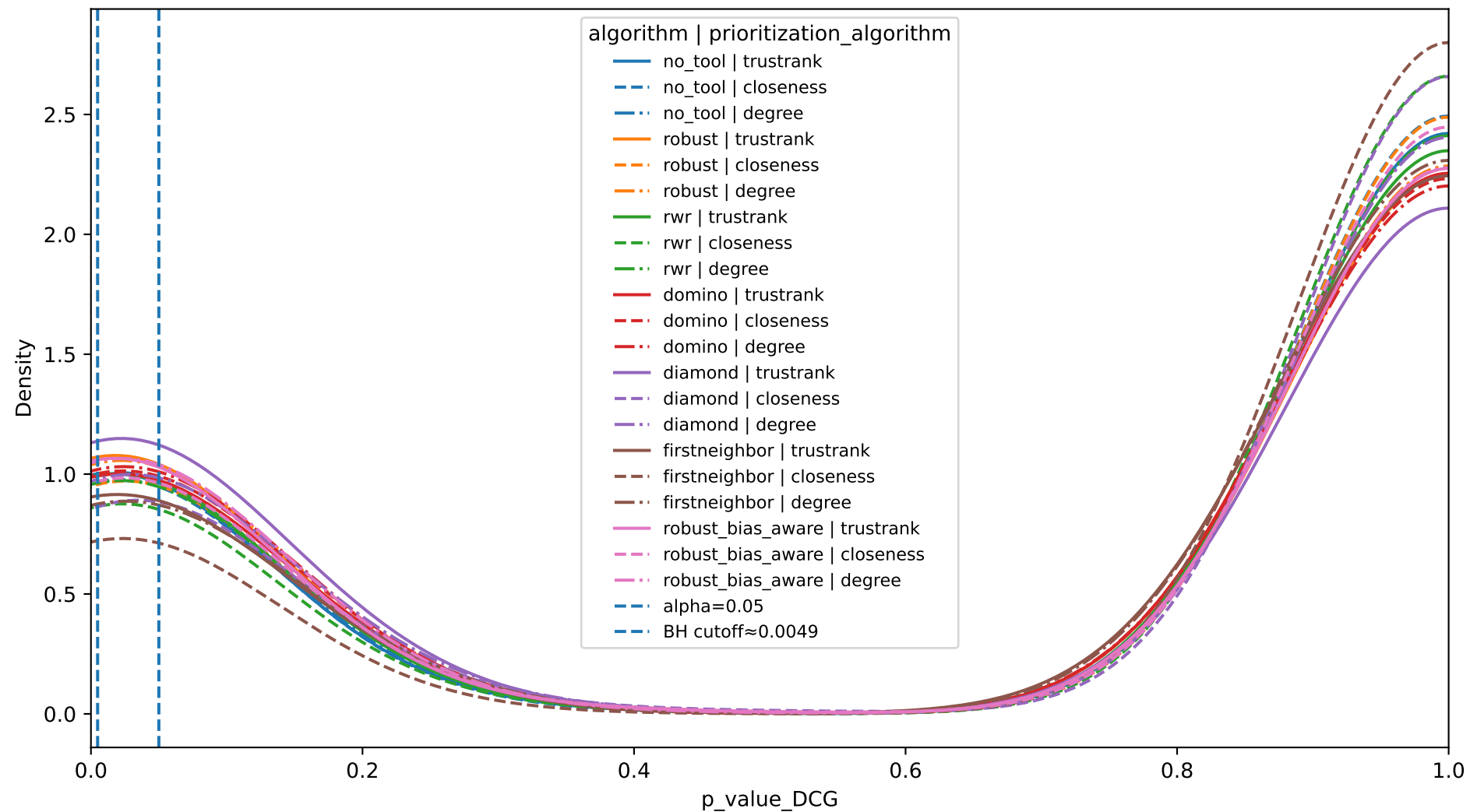
KDE of DCG p-values by algorithm and prioritization_algorithm (string_min700)
