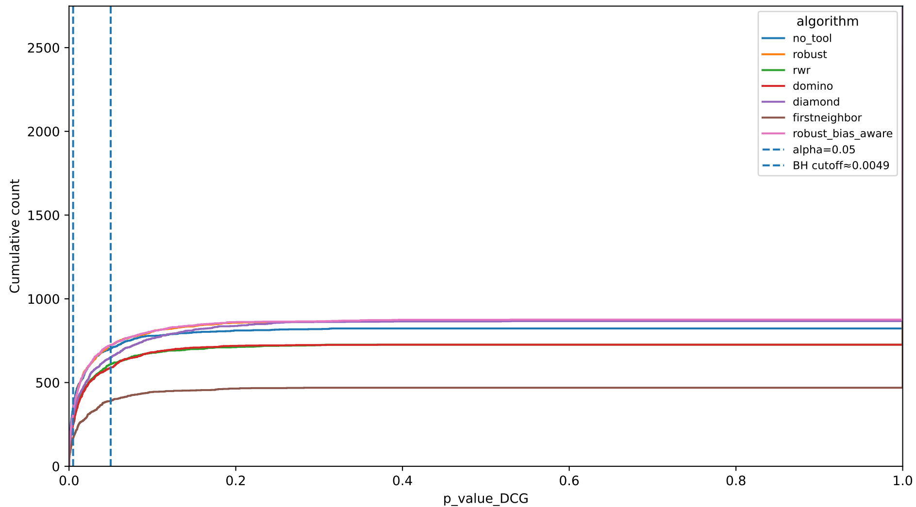
Cumulative count of DCG p-values by algorithm (string_min700)
