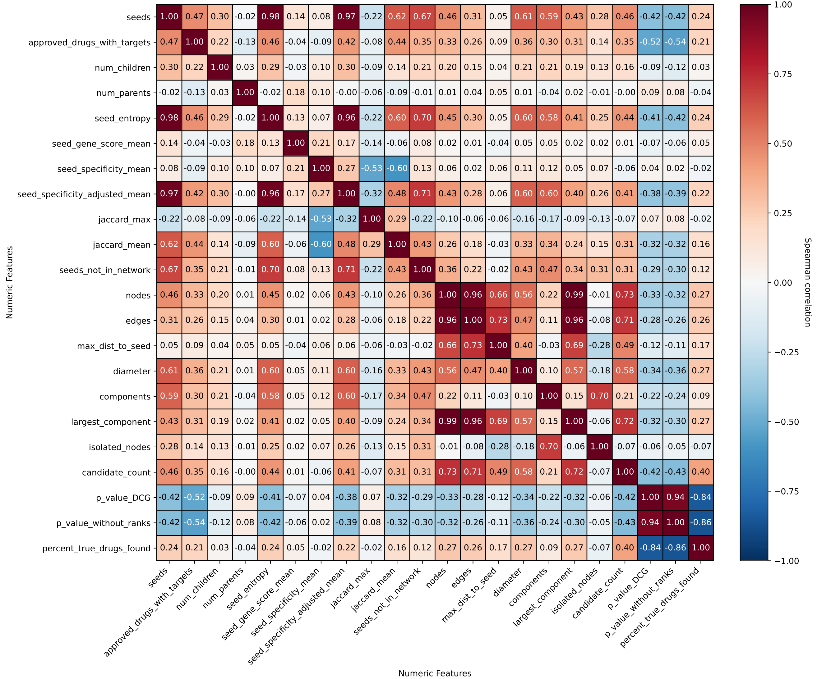
Correlation Heatmap of Numeric Metrics (best per sample) (string_min700)
