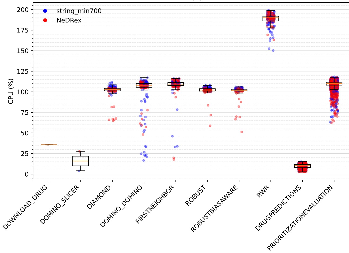
CPU (%) by process
