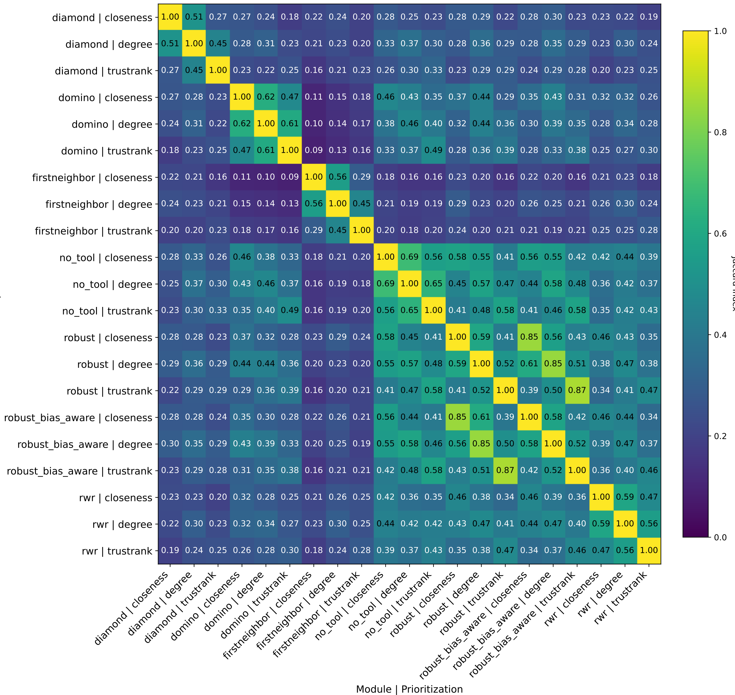
Jaccard Index Matrix (significant results) (string_min700)
