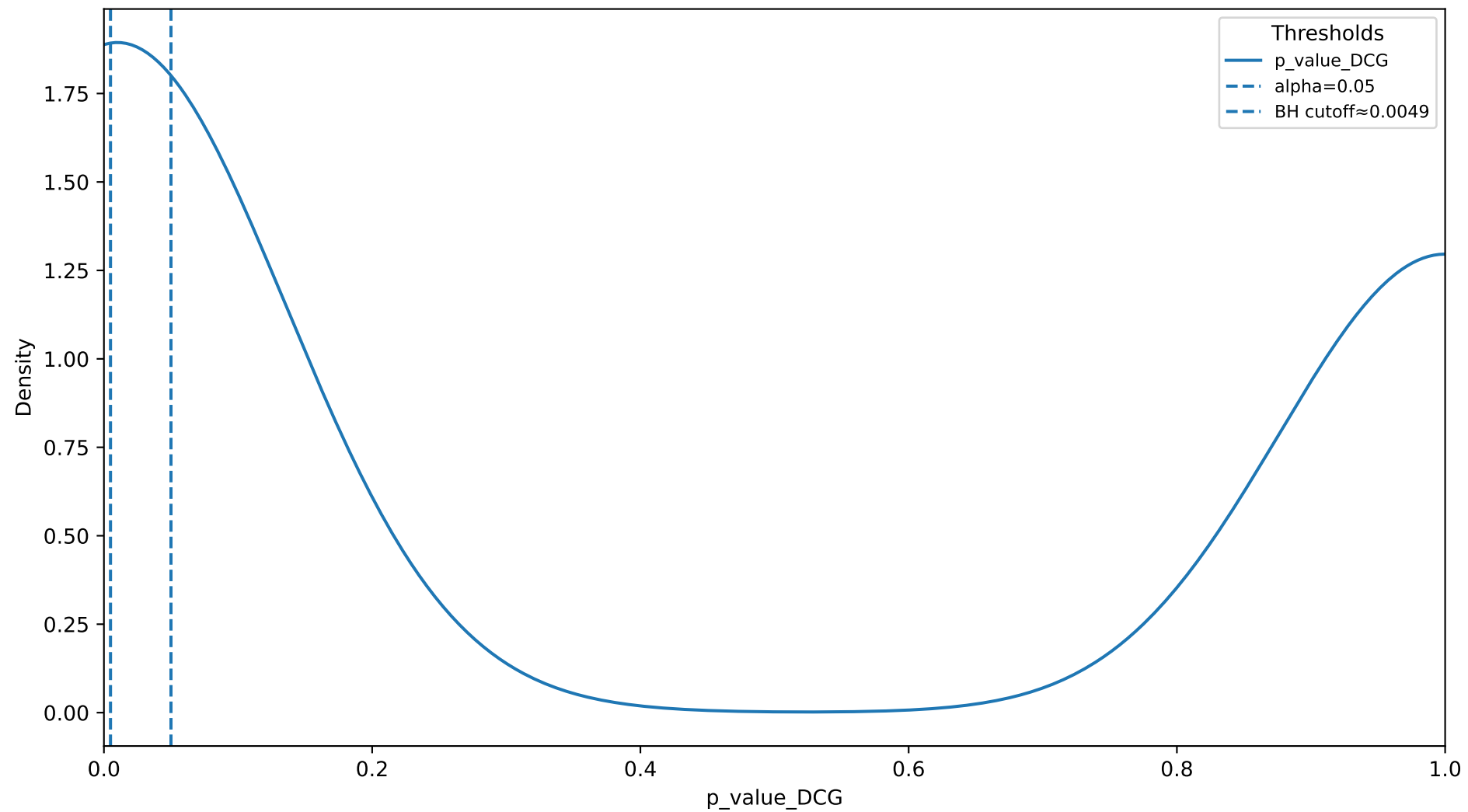
KDE of DCG p-values (best per sample, including p=1) (string_min700)
