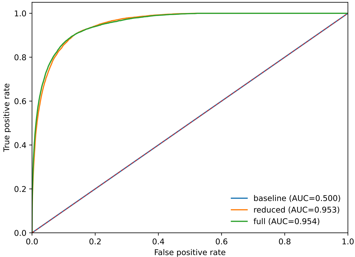
ROC curves
