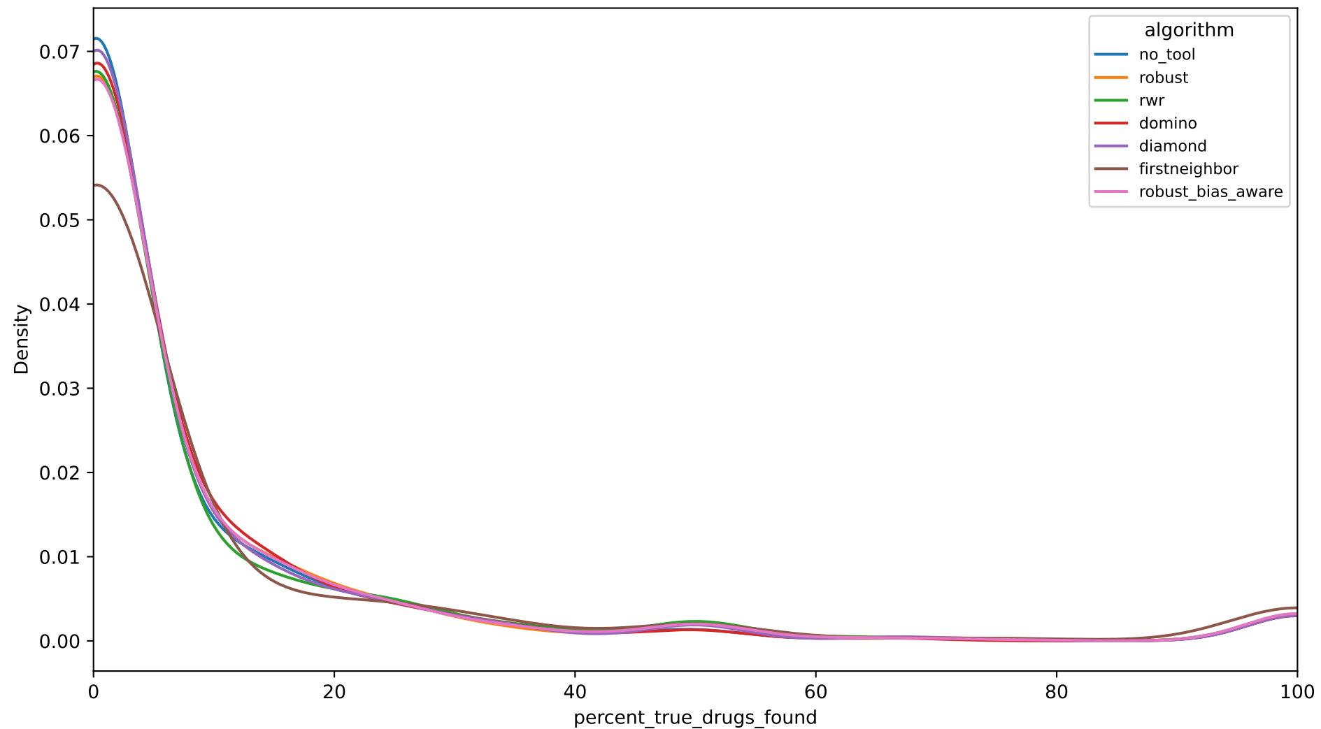
KDE of percent true drugs found by algorithm (string_min700)
