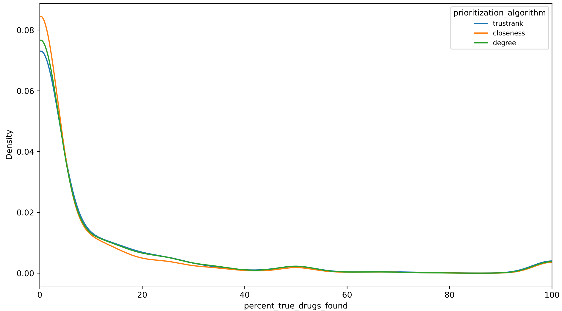
KDE of percent true drugs found by prioritization_algorithm (string_min700)
