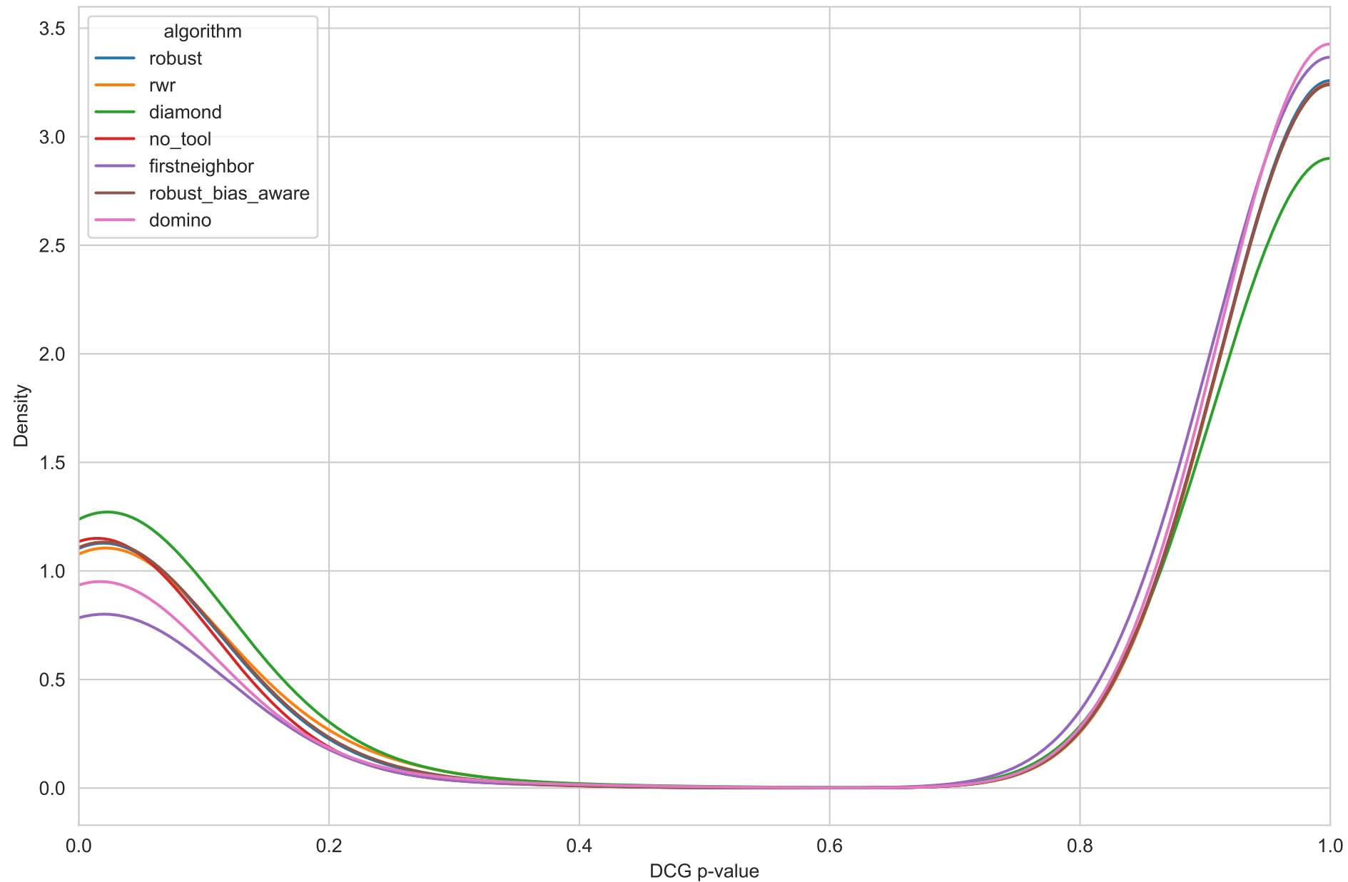
KDE of DCG p-values by algorithm
