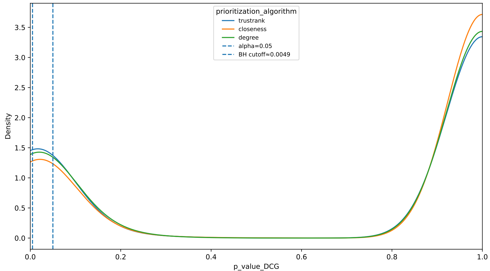
KDE of DCG p-values by prioritization_algorithm (string_min700)
