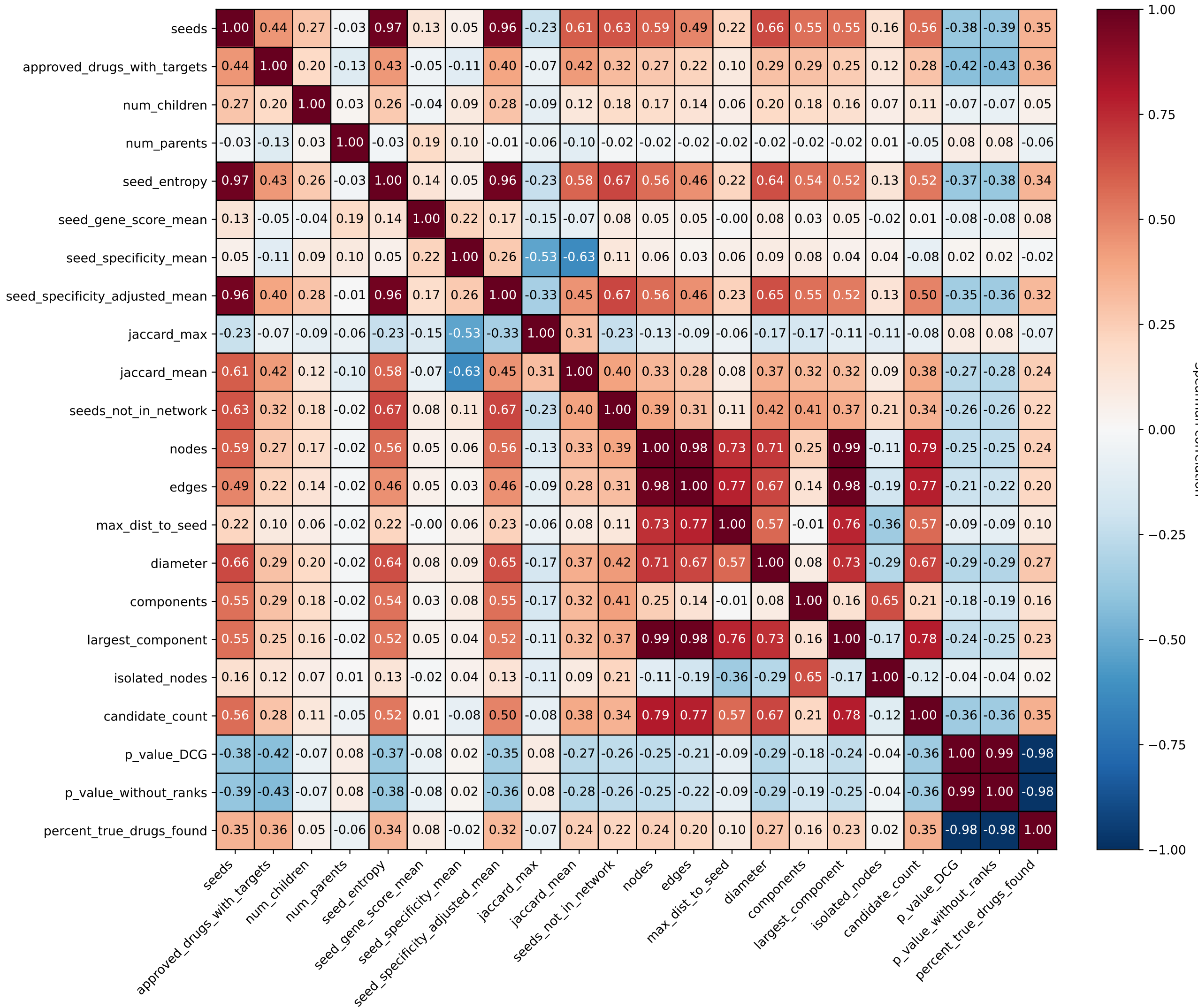
Correlation Heatmap of Numeric Metrics (string_min700)
