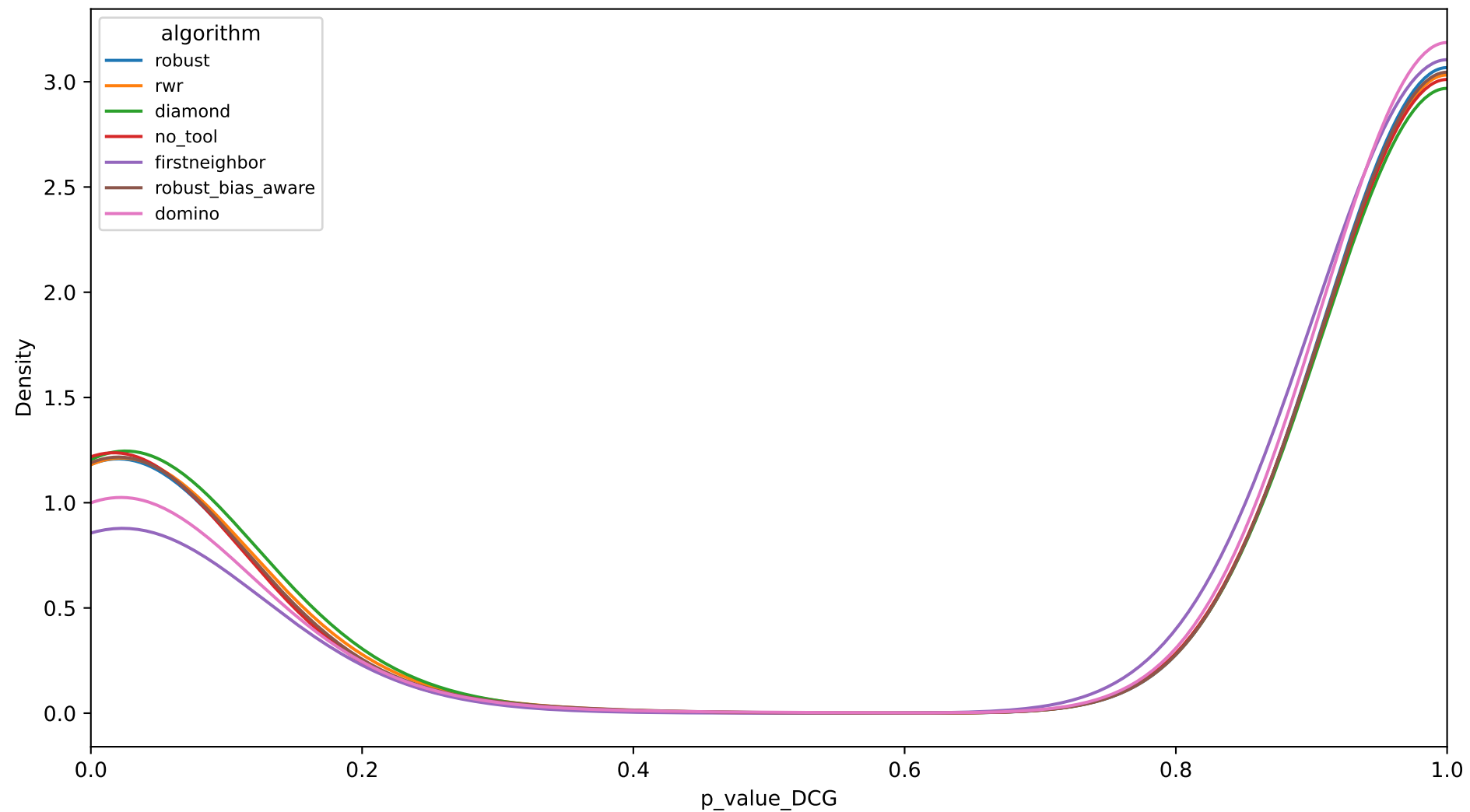
KDE of DCG p-values by algorithm (NeDRex)
