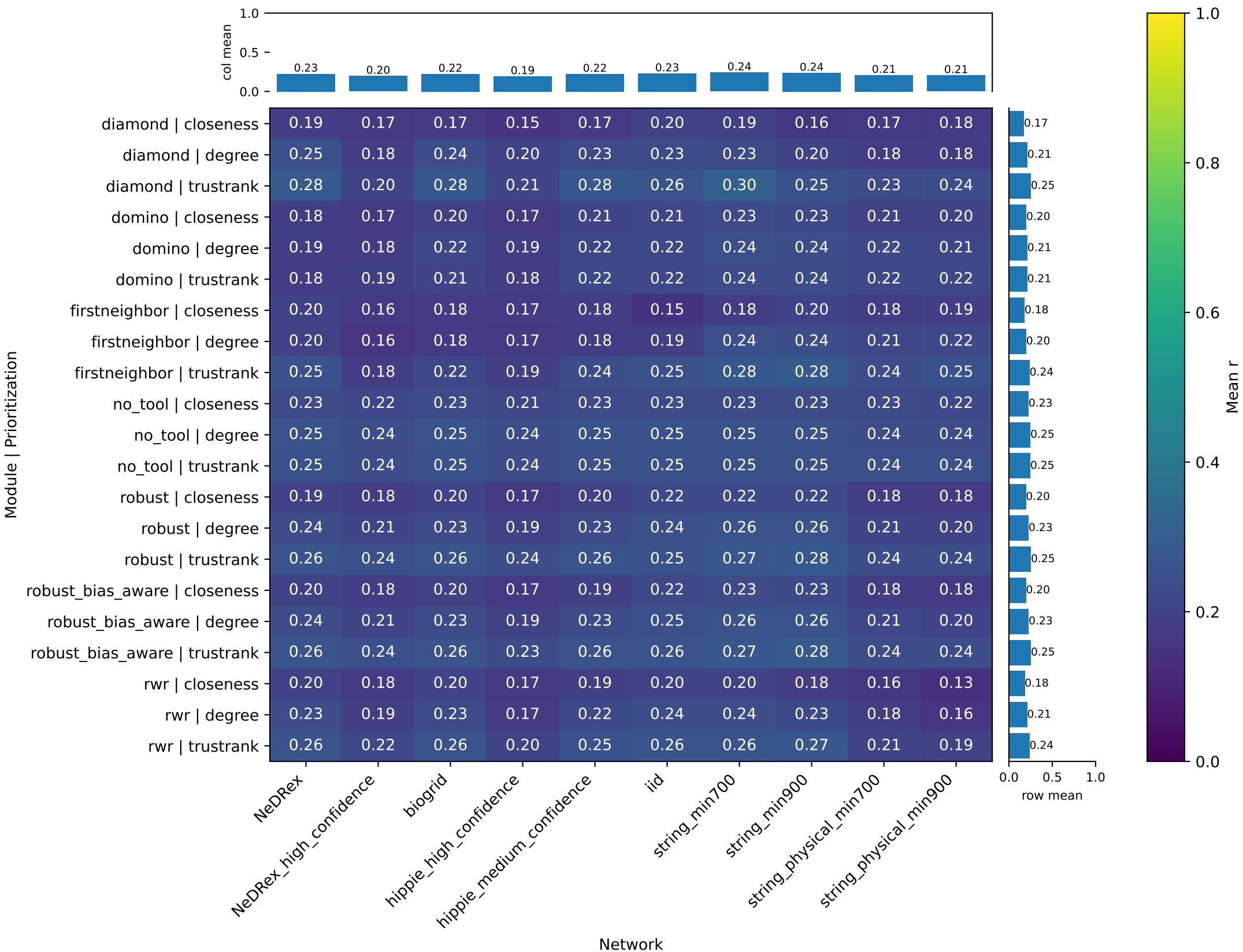
Mean closeness-to-best ratio across ALL methods and networks ( r = \text{score} / \text{best score per disease} , \text{score} = -\log_{10} p )
