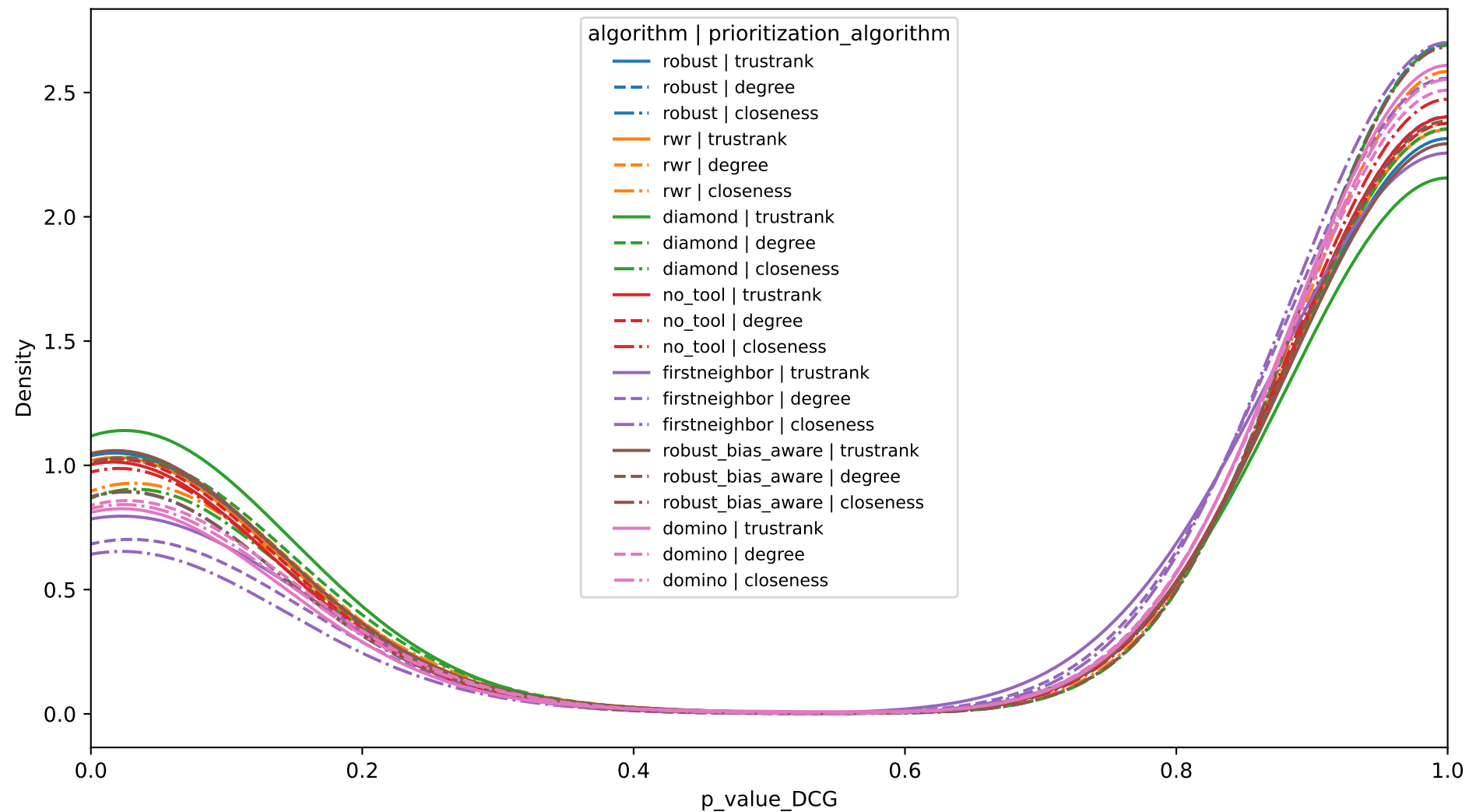
KDE of DCG p-values by algorithm and prioritization_algorithm (NeDRex)
