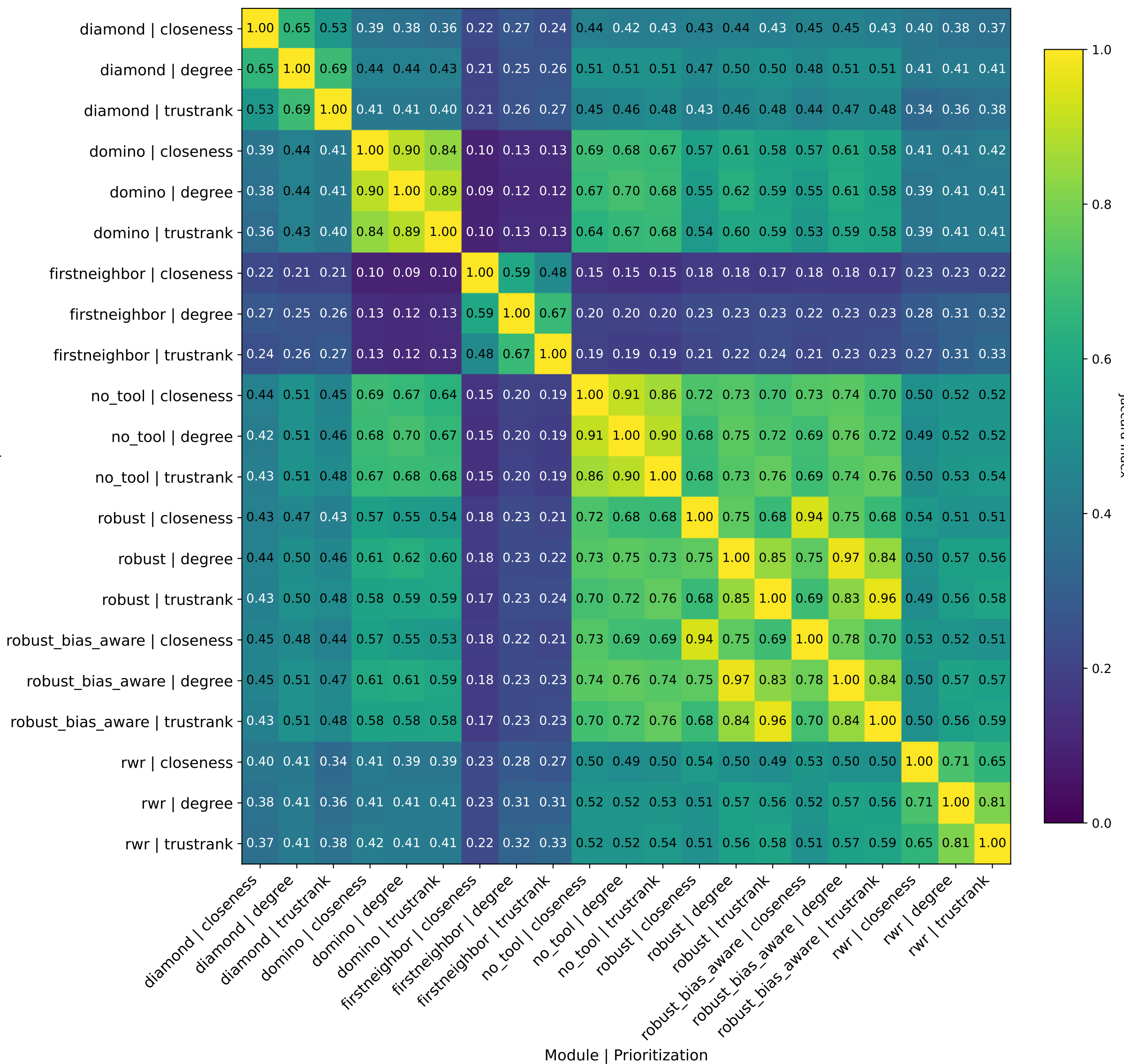
Jaccard Index Matrix(p_value_DCG &lt; 1) (string_min700)
