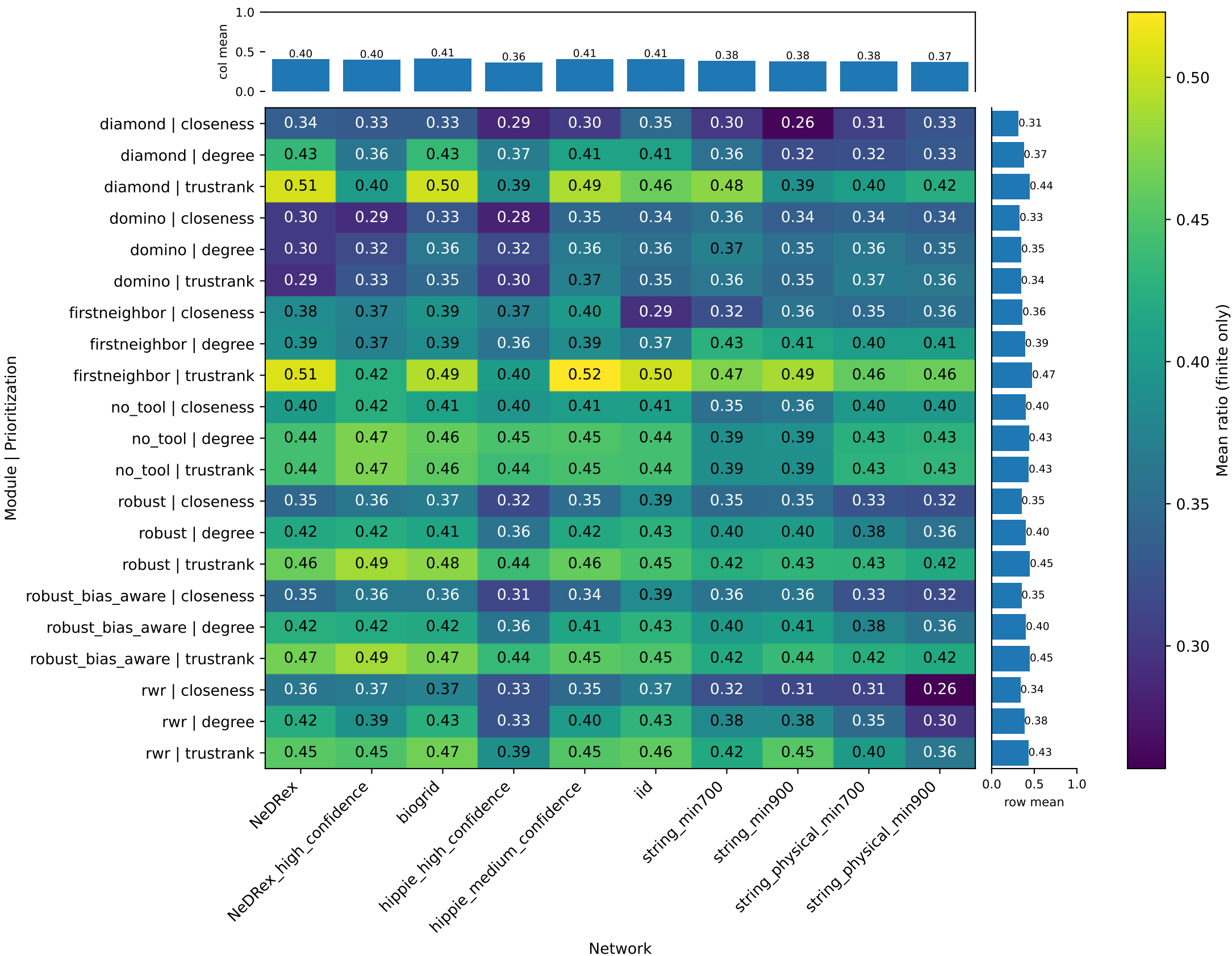
Mean score/best score ratio ( -\log_{10} p )
