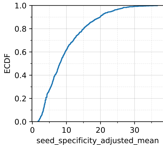
Empirical CDFs (unique per sample)
