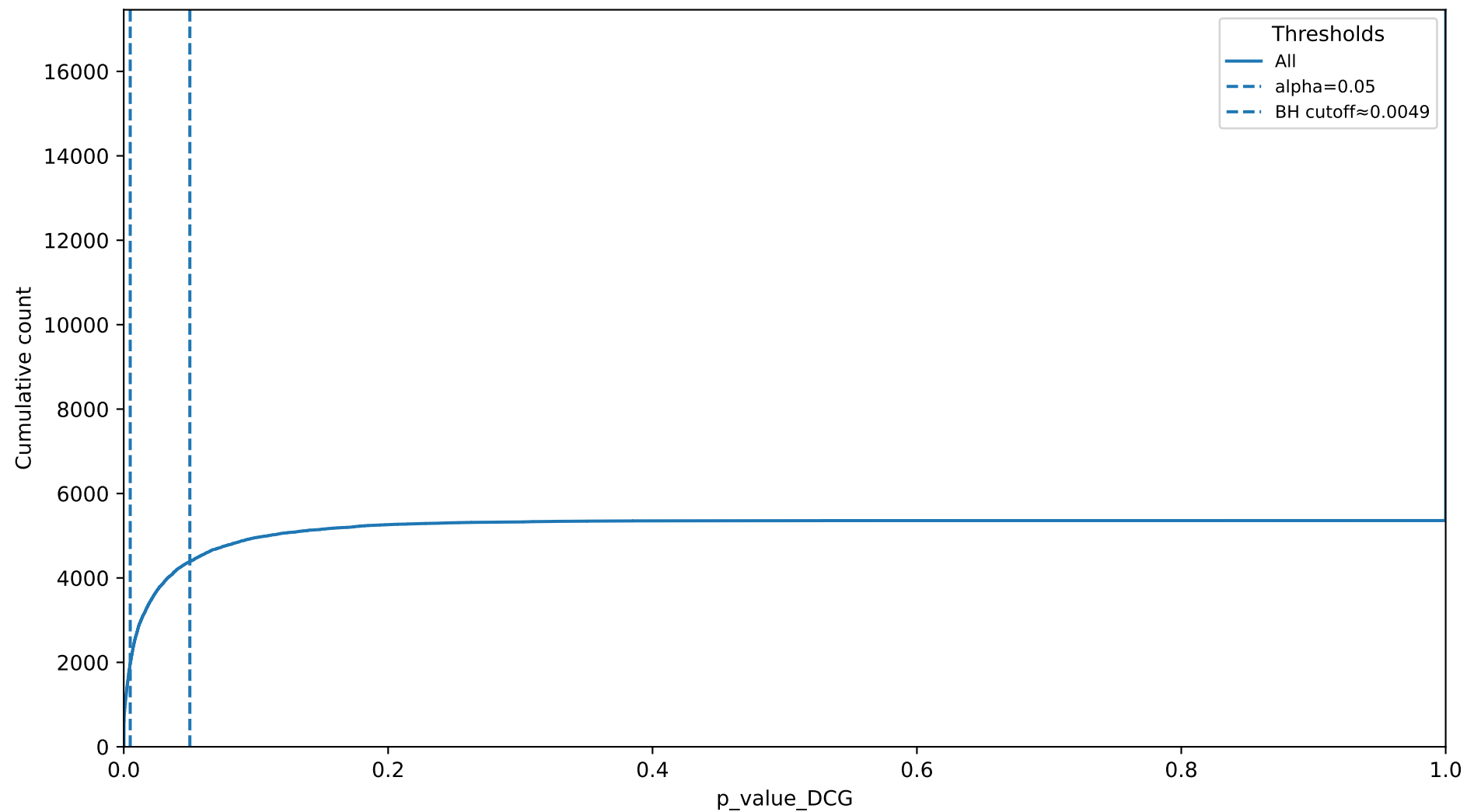
Cumulative count of DCG p-values (string_min700)
