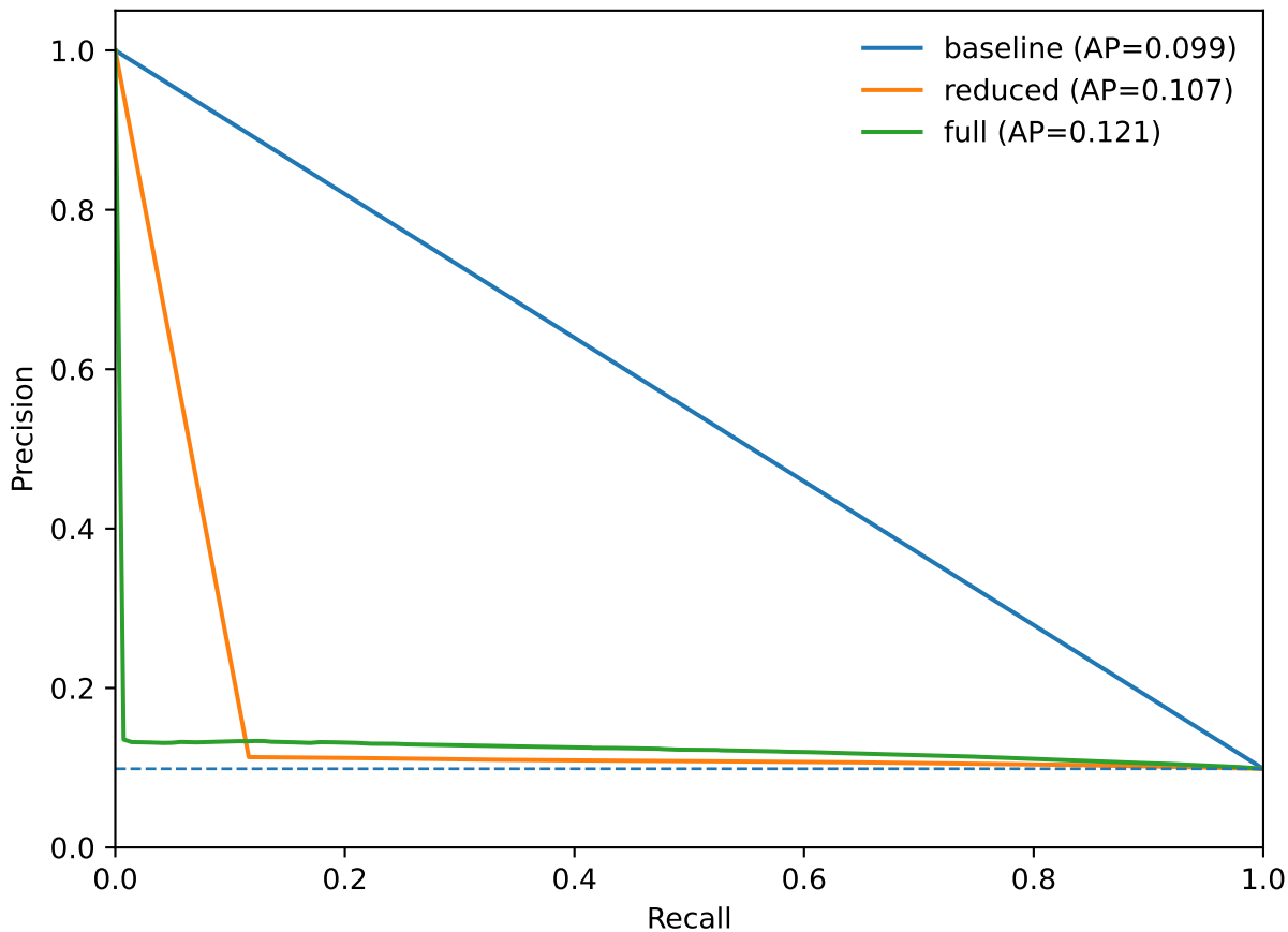
Precision-Recall curves
