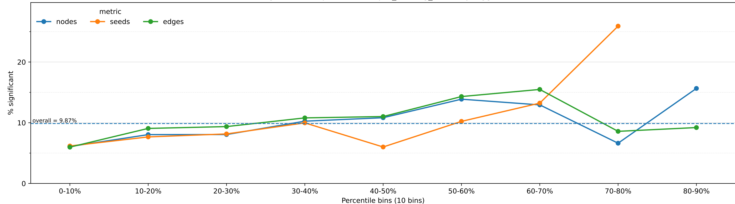
% significant vs quantile bins [per_row, sig_rule=any, agg=n/a]
