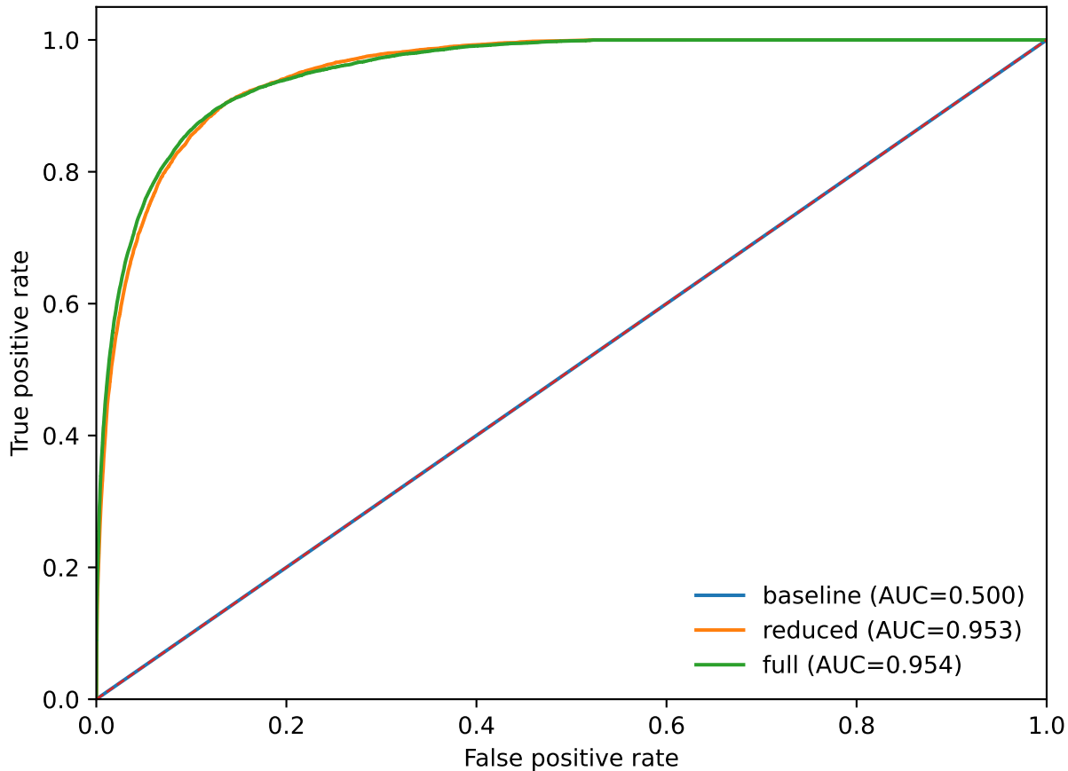
ROC curves
