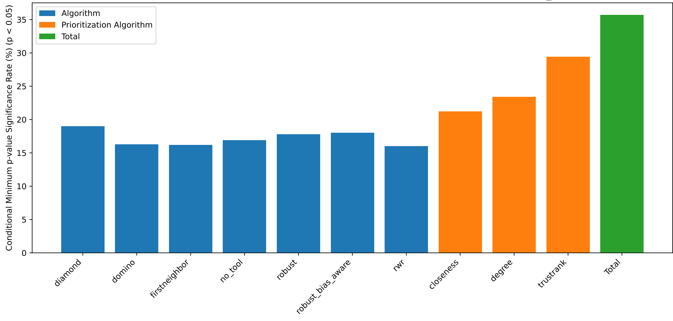
Minimum p-value Significance Rates by Category (Conditional on Delivered Results) (string_min700)
