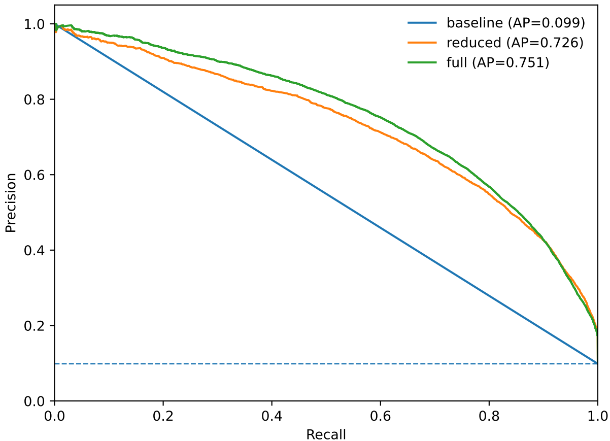
Precision-Recall curves
