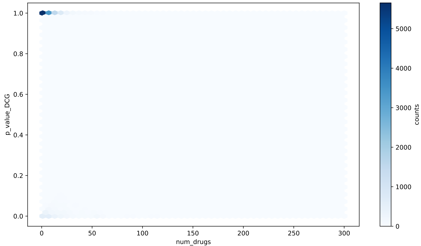
Hexbin of num_drugs vs p_value_DCG (string_min700)
