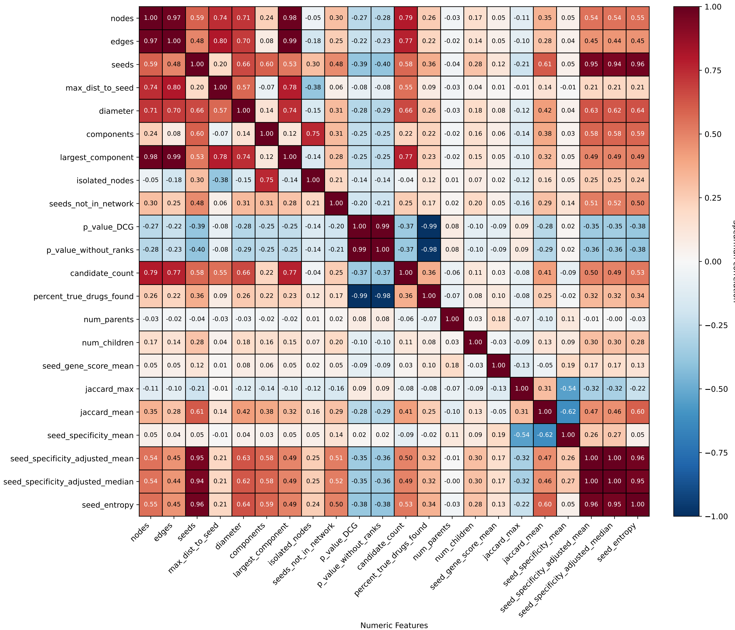
Correlation Heatmap of Numeric Metrics (NeDRex)
