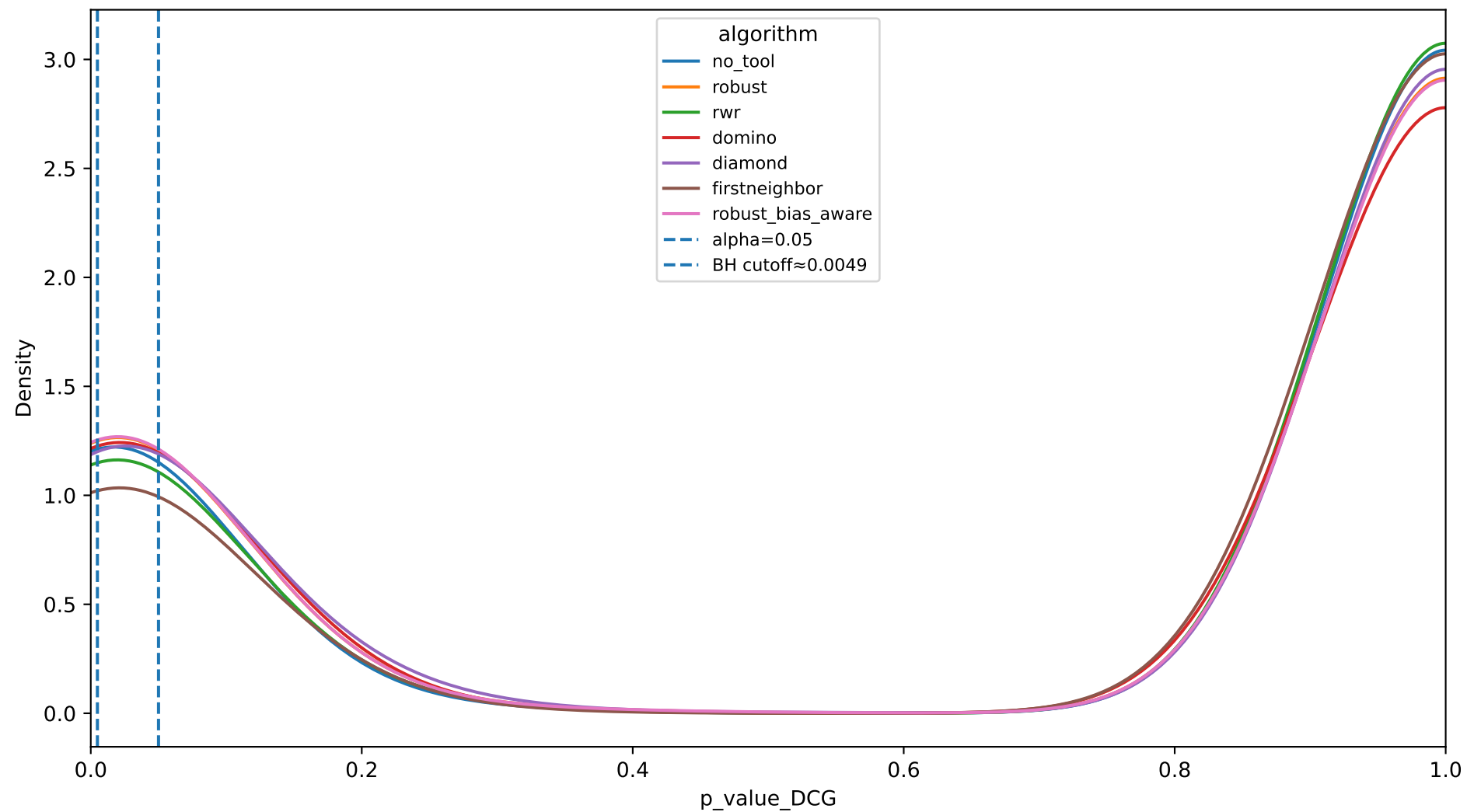
KDE of DCG p-values by algorithm (string_min700)
