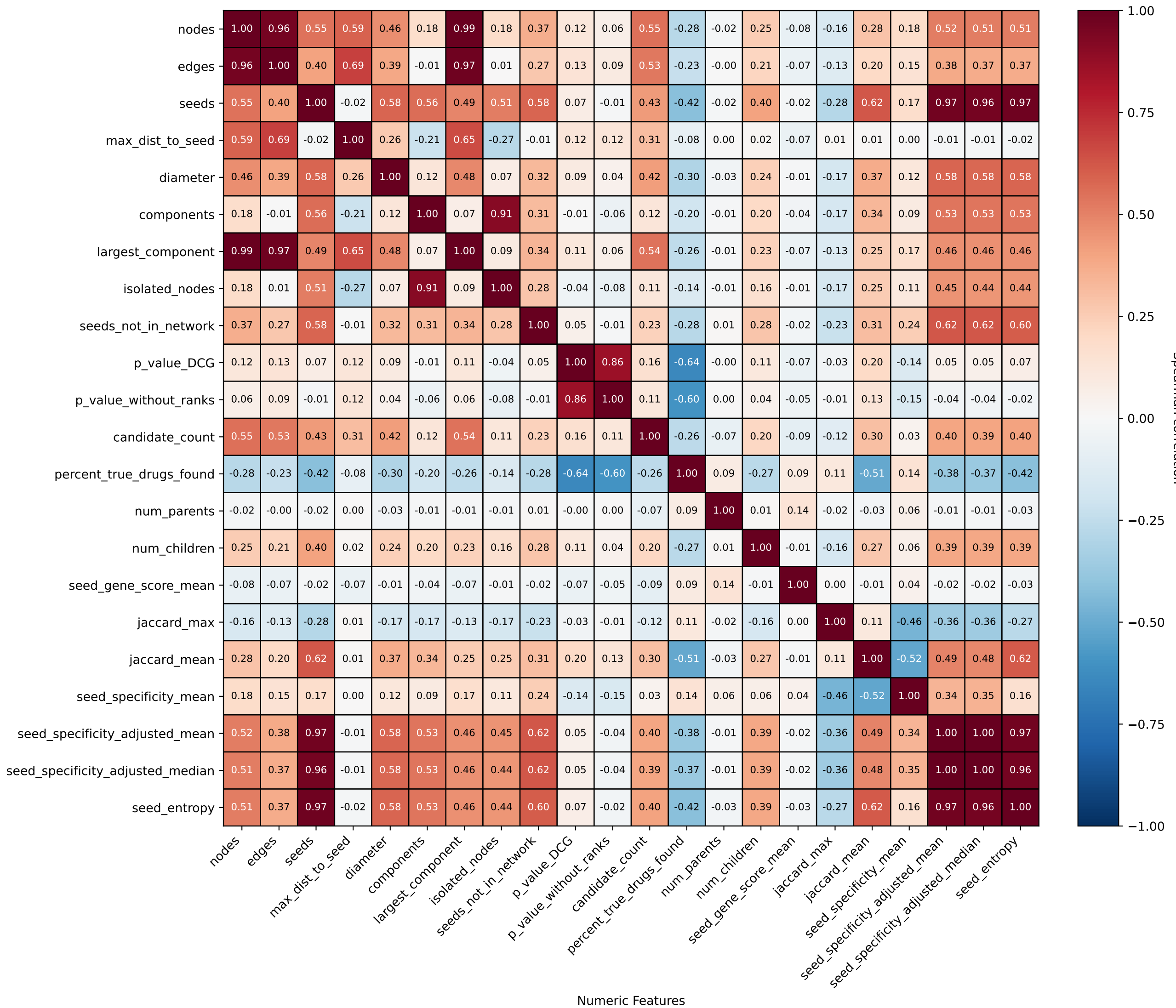
Correlation Heatmap of Numeric Metrics, excluding p_value_DCG = 1 (NeDRex)
