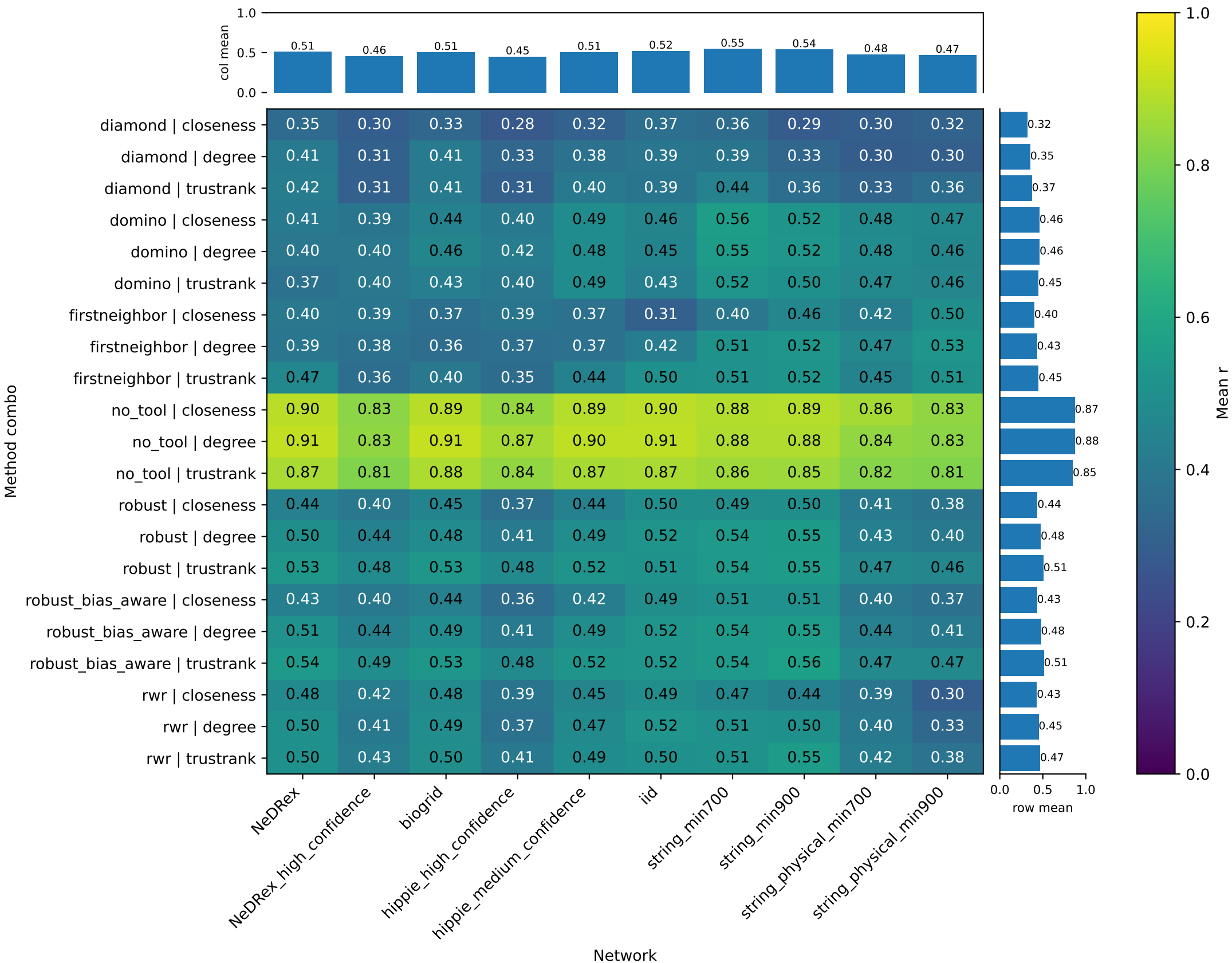
Row-wise mean r across networks per method (r = score/best within method)
