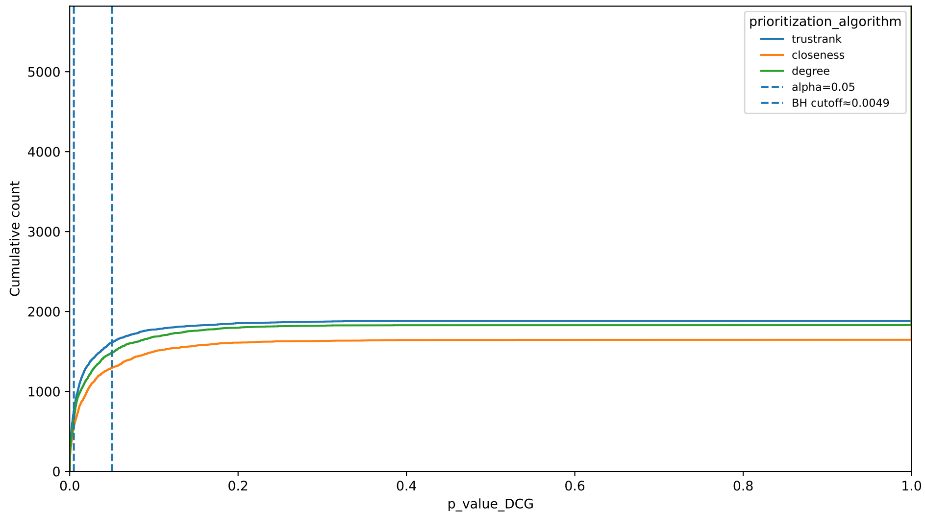
Cumulative count of DCG p-values by prioritization_algorithm (string_min700)
