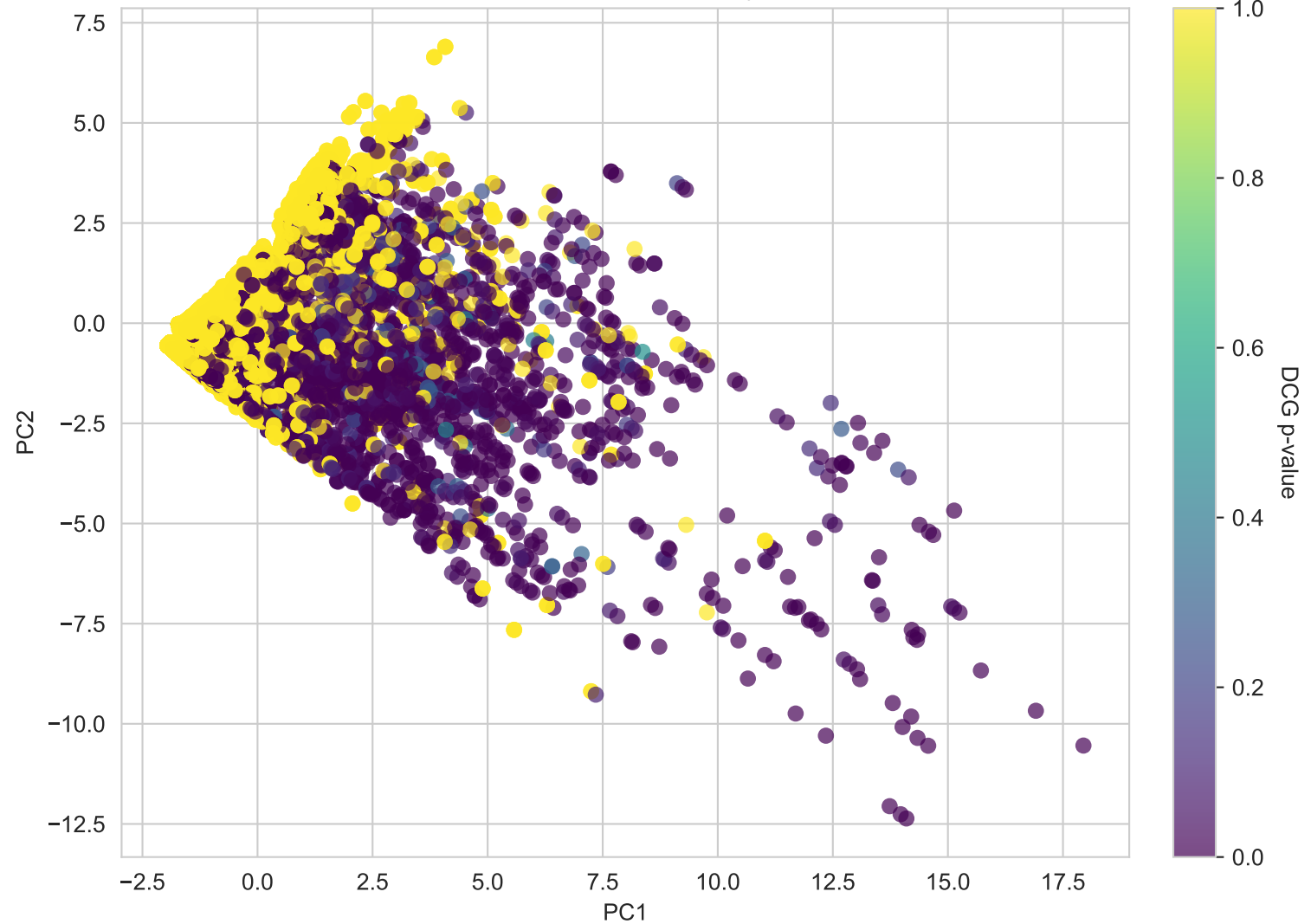
PCA of Numeric Metrics Colored by DCG p-value
