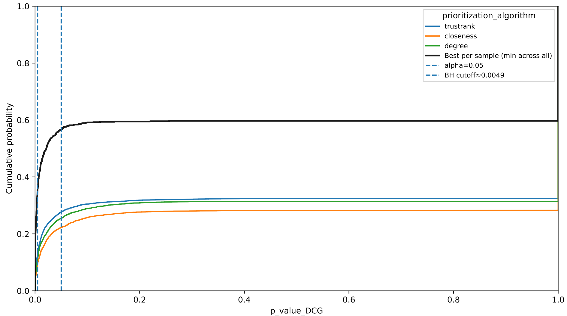
ECDF of DCG p-values by prioritization_algorithm (string_min700)
