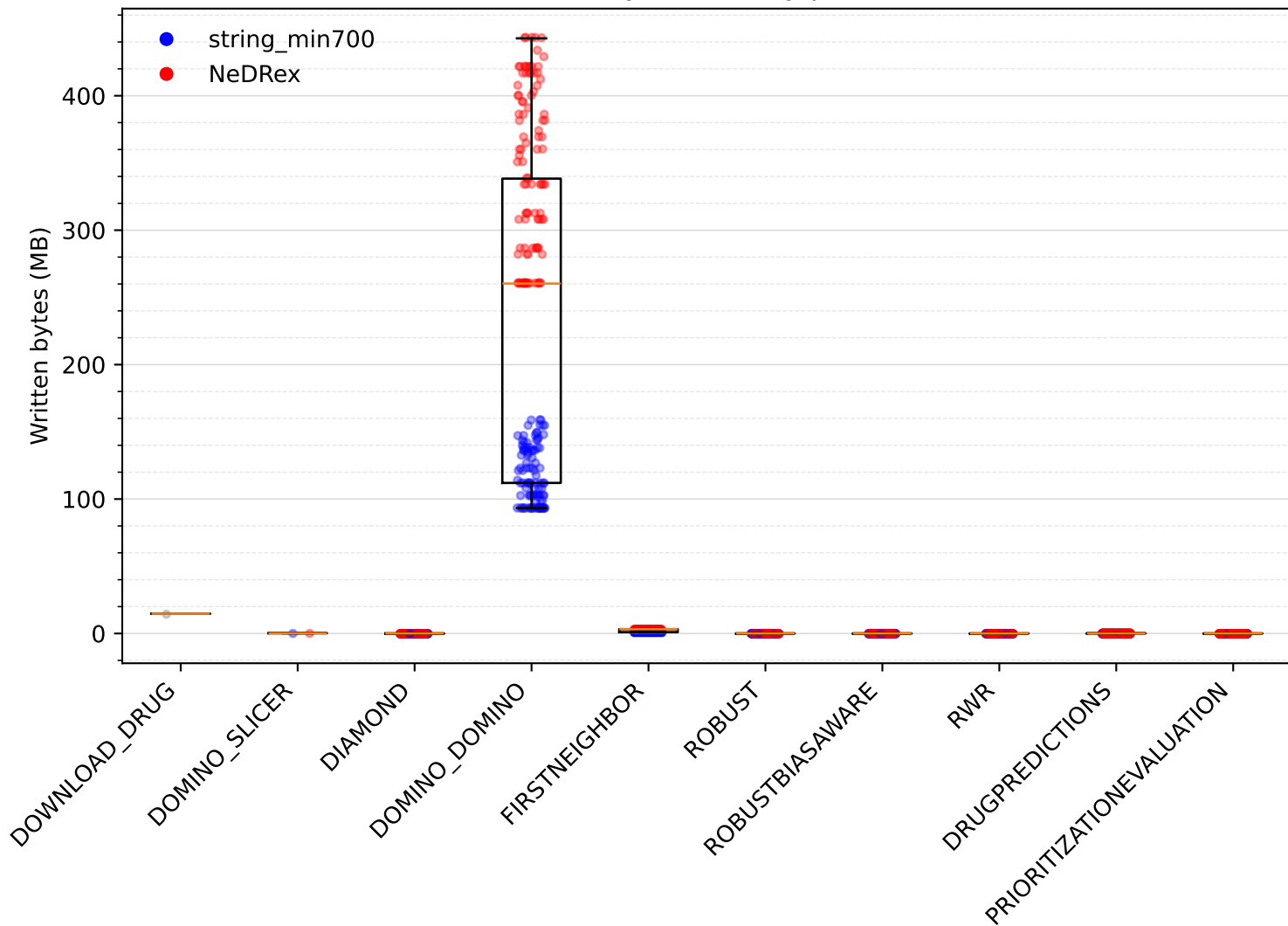
Written bytes (MB) by process
