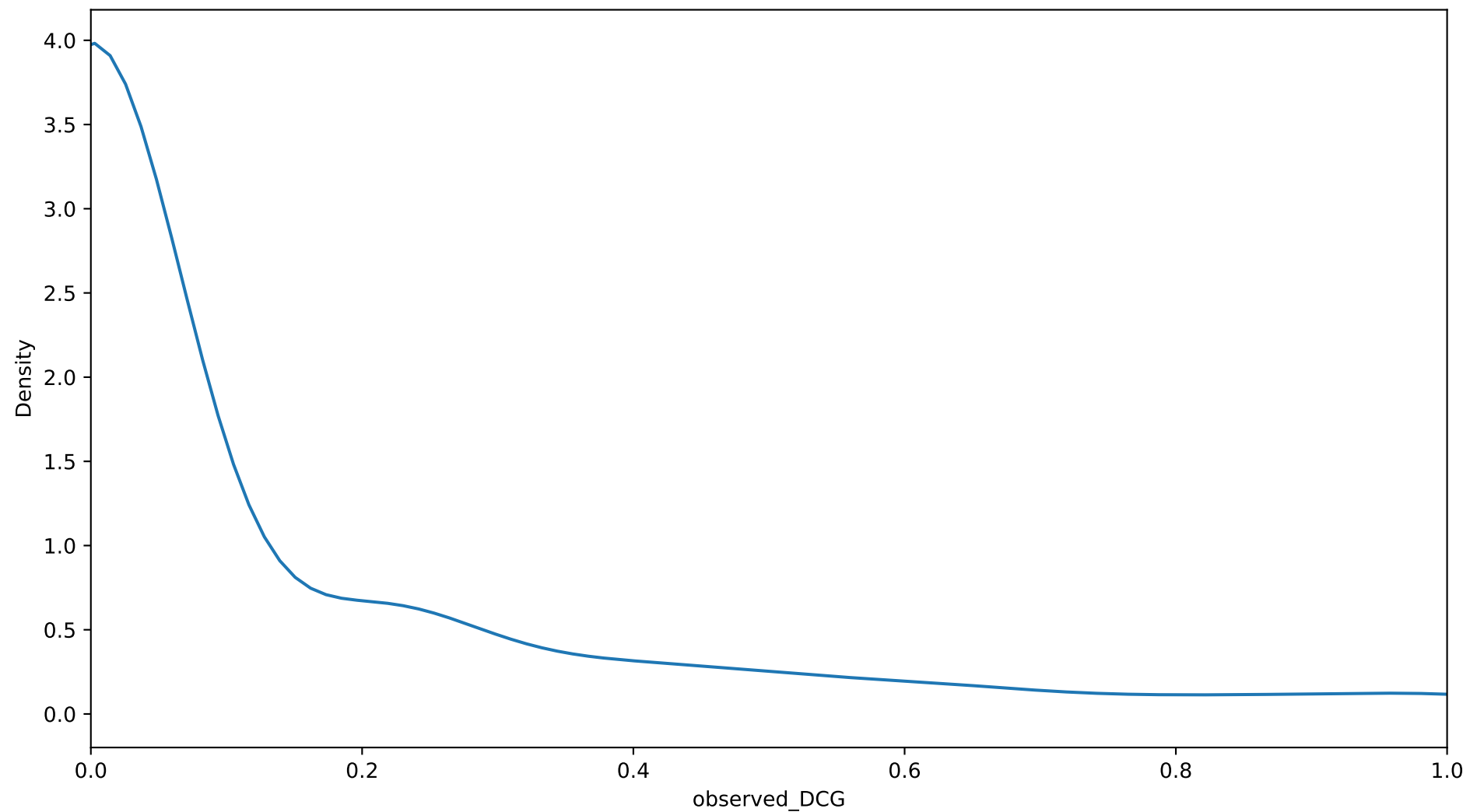
KDE of Observed DCG (string_min700)
