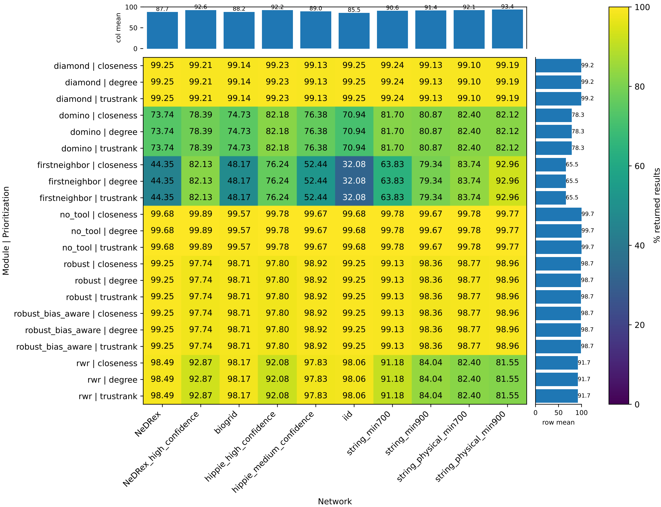
Coverage: percent of diseases with a returned result by method × network Denominator = unique diseases per network; Numerator = diseases where the method returned any result
