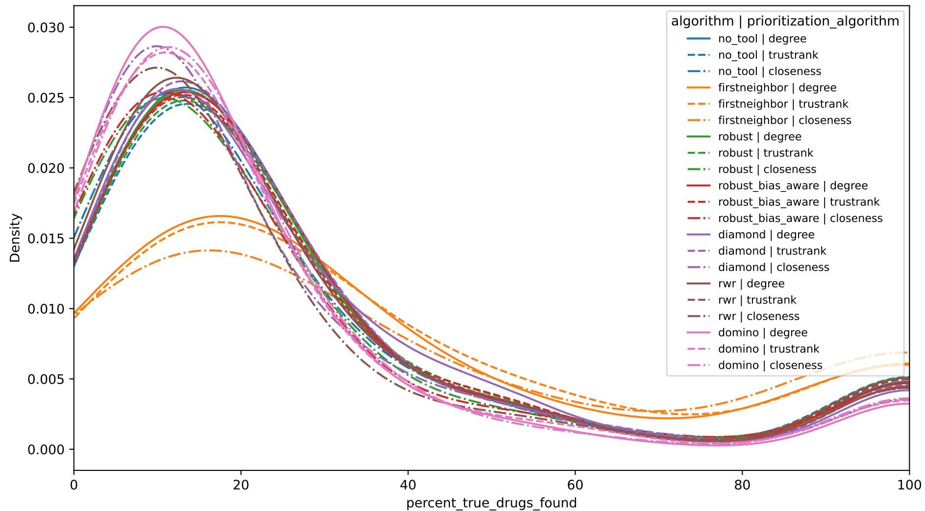
KDE of percent true drugs found by algorithm and prioritization_algorithm, excluding 0 (NeDRex)
