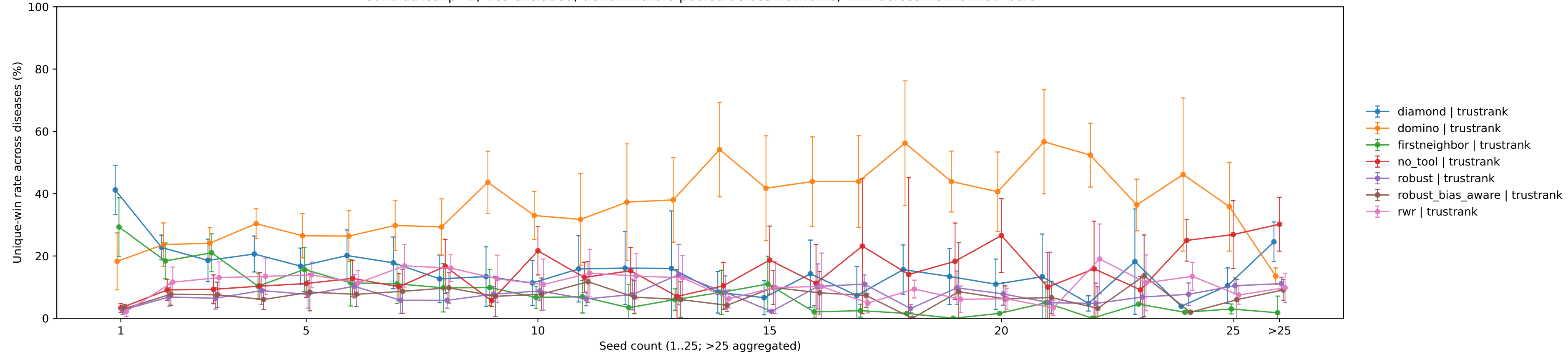
TrustRank-only: pooled unique-win rate vs seed count across networks Candidates: p < 1 ; ties excluded; denominators pooled across networks; with across-network SD bars
