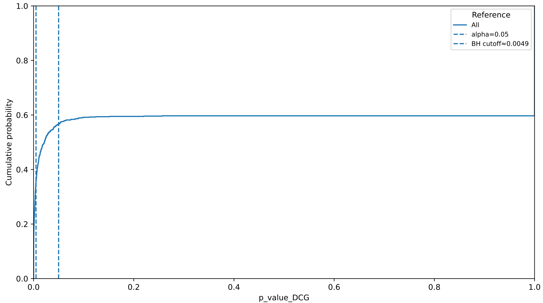
ECDF of DCG p-values (best per sample, including p=1) (string_min700)
