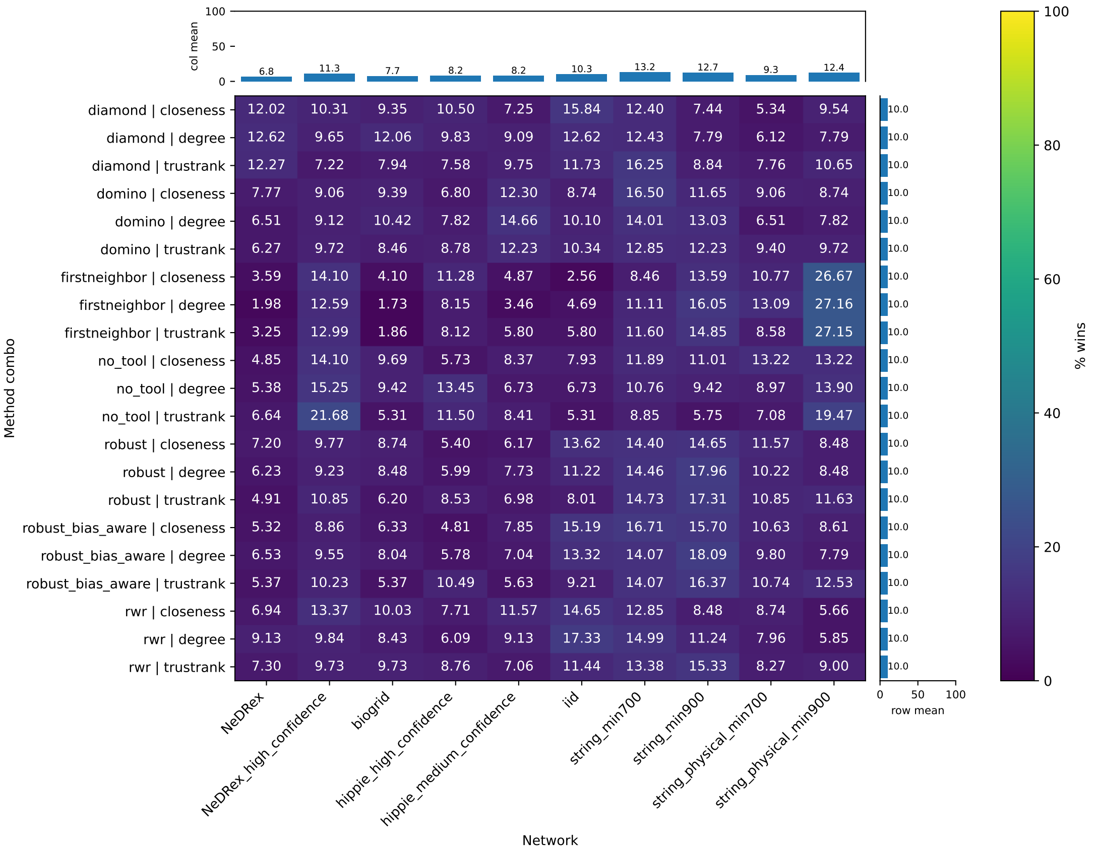
Row-wise network win rate per method (unique min p, p=1 excluded)
