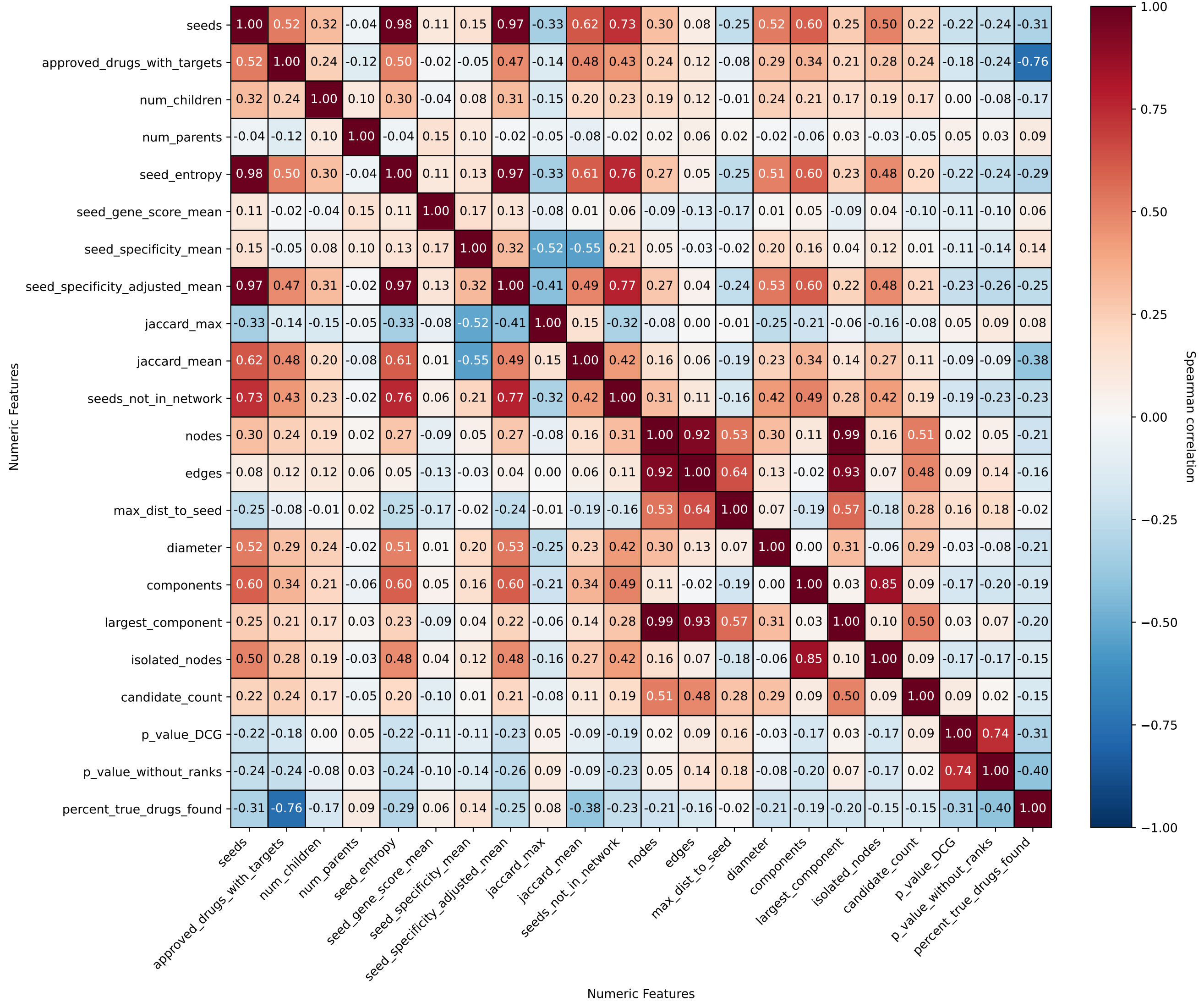
Correlation Heatmap of Numeric Metrics (best per sample, excluding p_value_DCG = 1) (string_min700)
