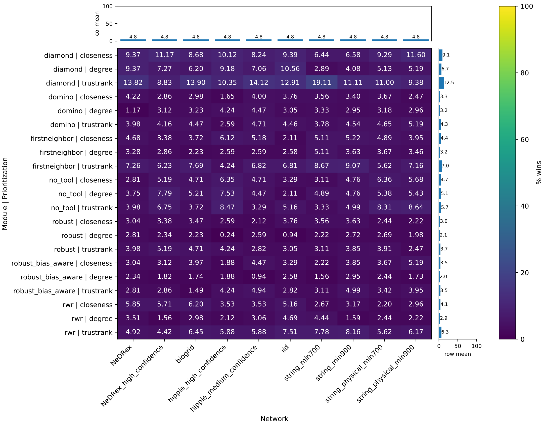
Win rate: % lowest p_value_DCG (excluding p=1 and ties)
