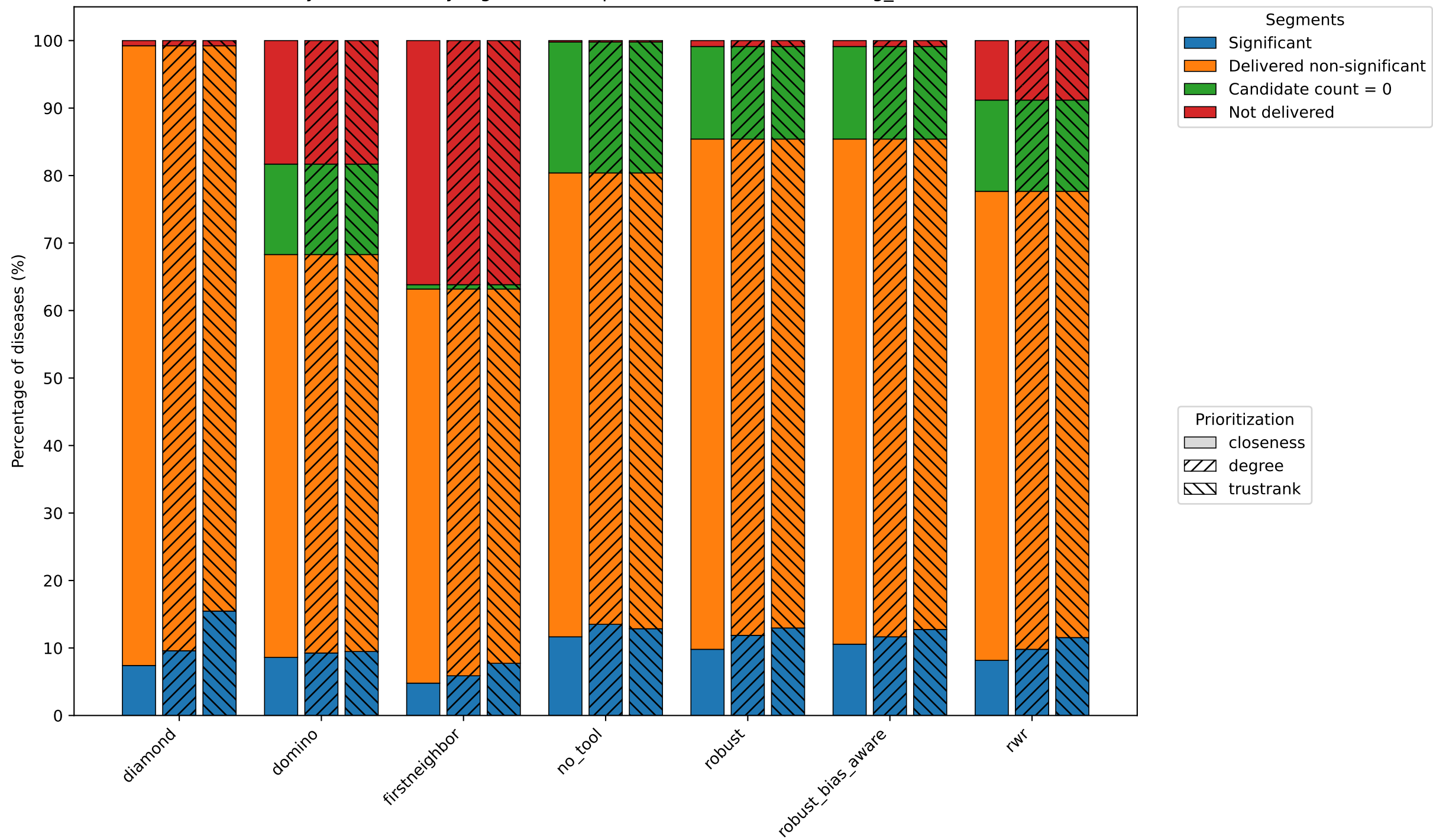
Delivery breakdown by algorithm and prioritization (stacked) (string_min700)
