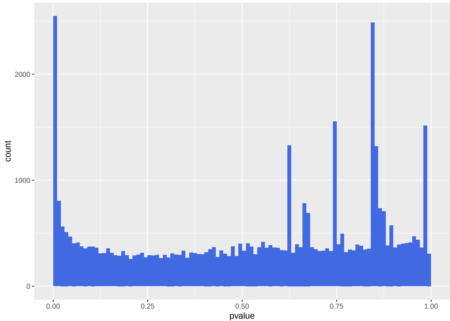
p-value distribution for star
