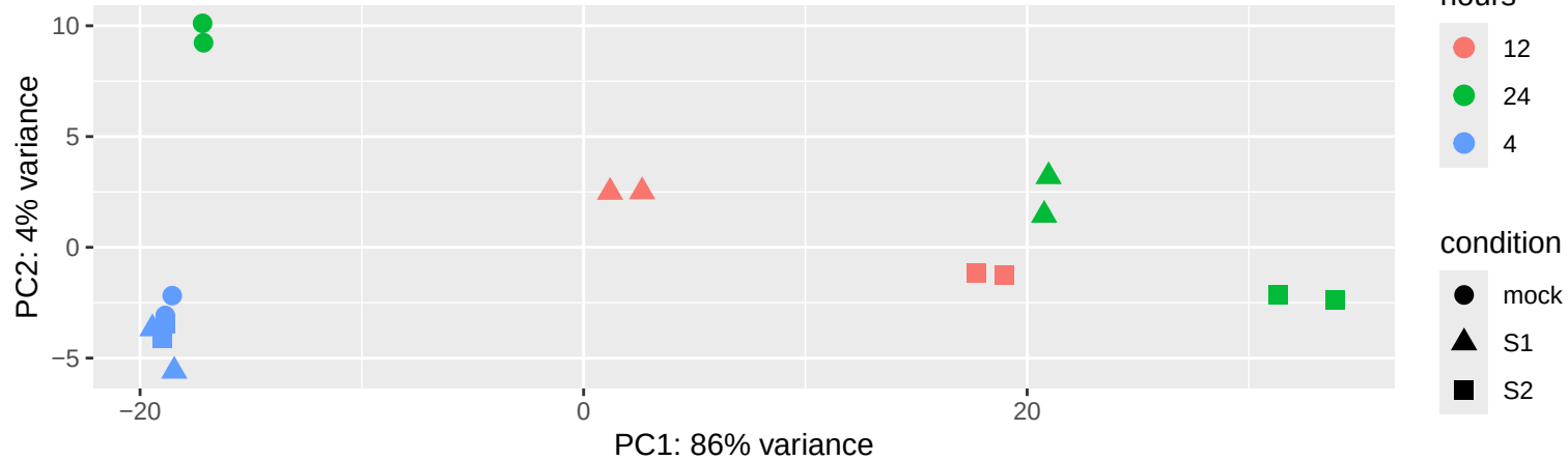
PCA Plot for hisat Analysis
