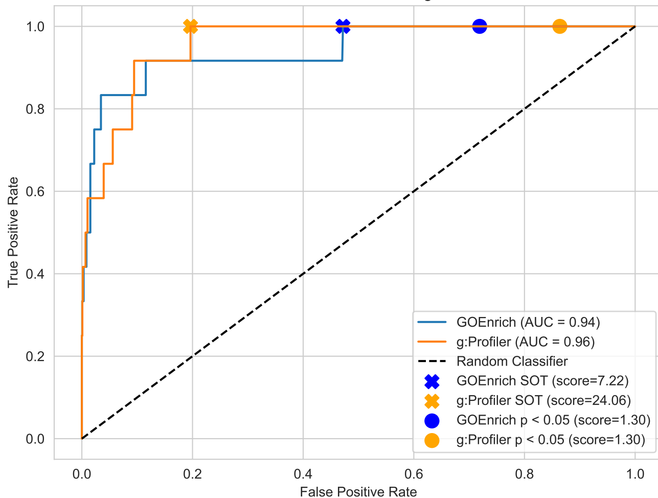
ROC Curve: GOEnrich vs. g:Profiler
