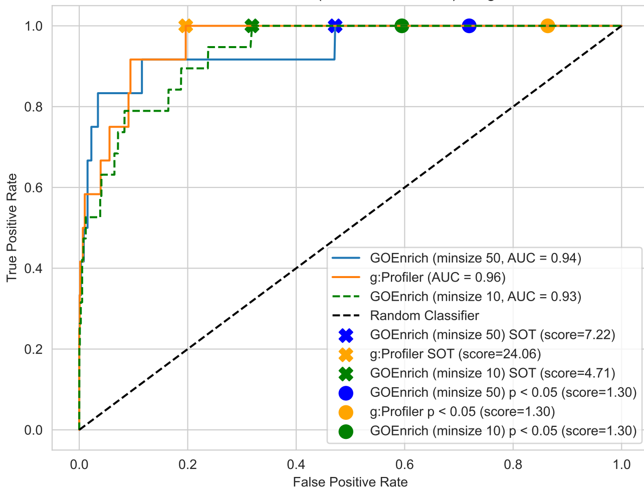
ROC Curve: GOEnrich (minsize 50 and 10) vs. g:Profiler
