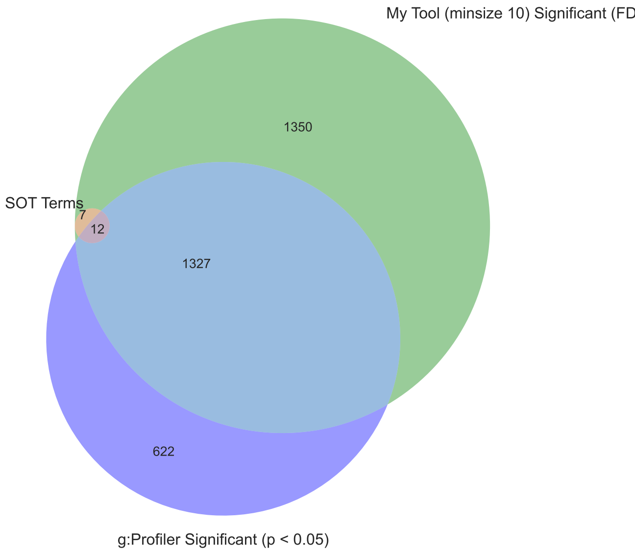
Venn Diagram: SOT vs. Significant GO Terms (My Tool minsize 10 vs. g:Profiler)
