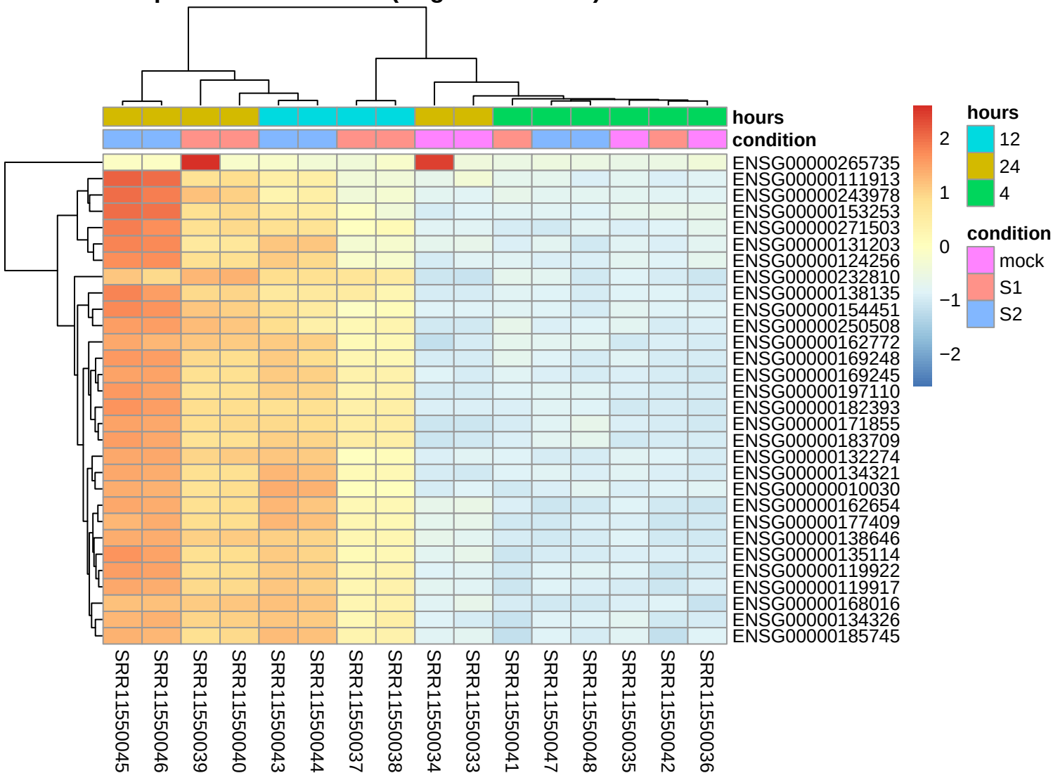
Top 30 Variable Genes (rlog transformed) for hisat
