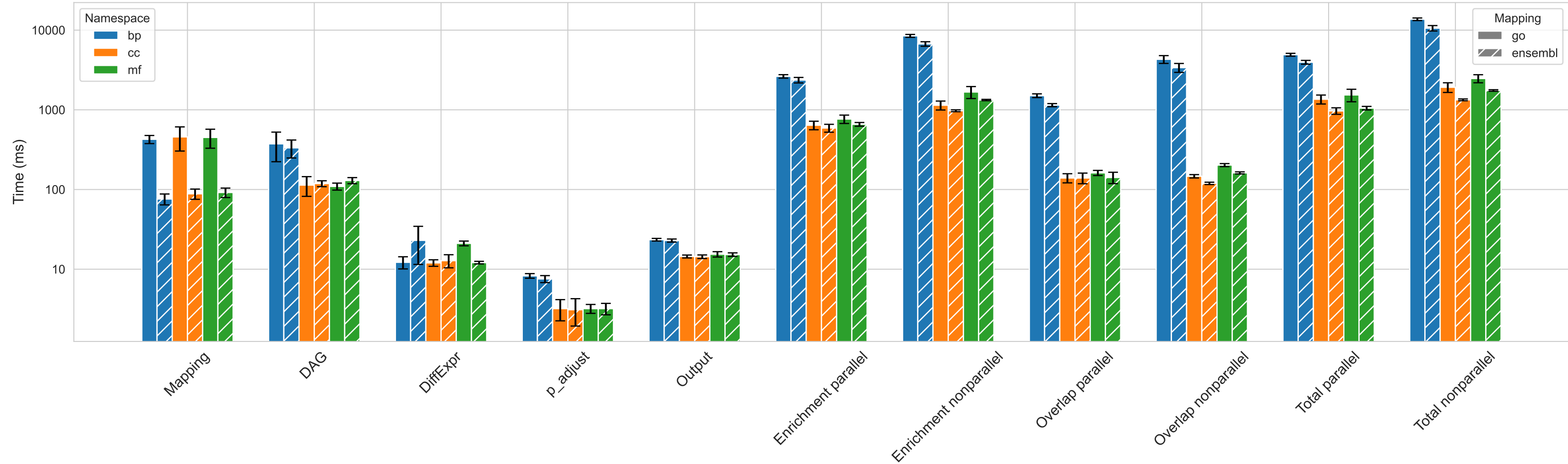
Runtime Breakdown by Category (Common Metrics & Jar-Specific (Split by Parallel))
