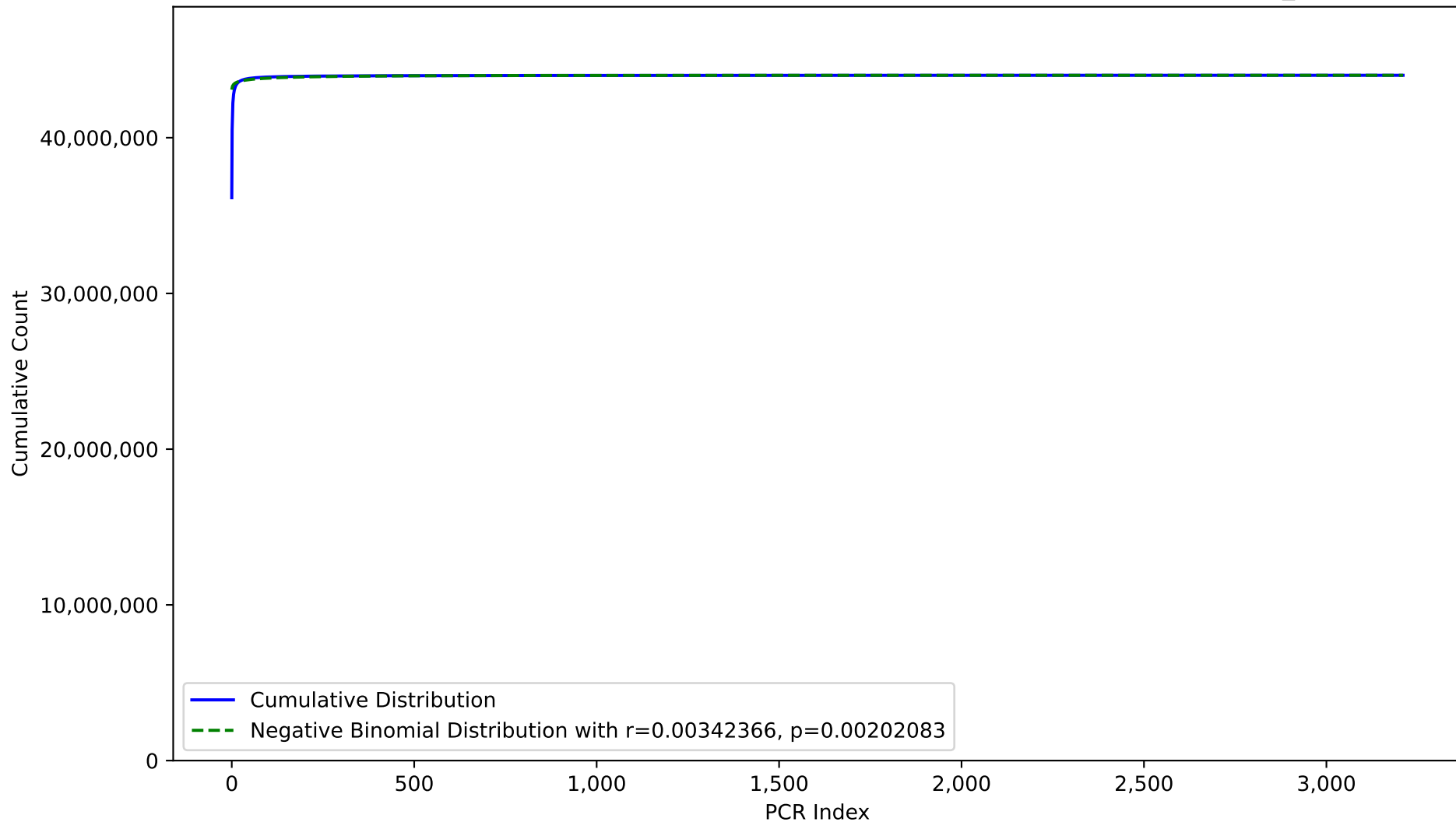
Cumulative Distribution of PCR Index Counts with Negative Binomial Fit for ebna_hisat
