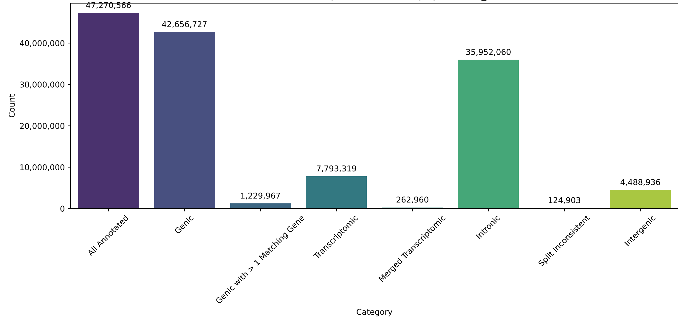
Number of Reads by Annotation Category for ebna_hisat
