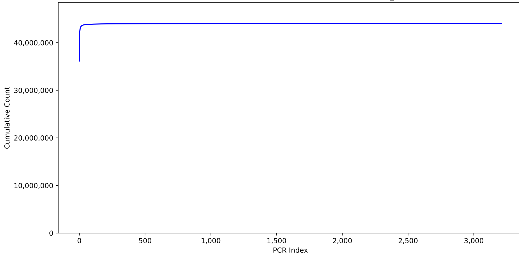
Cumulative Distribution of PCR Index Counts for ebna_hisat
