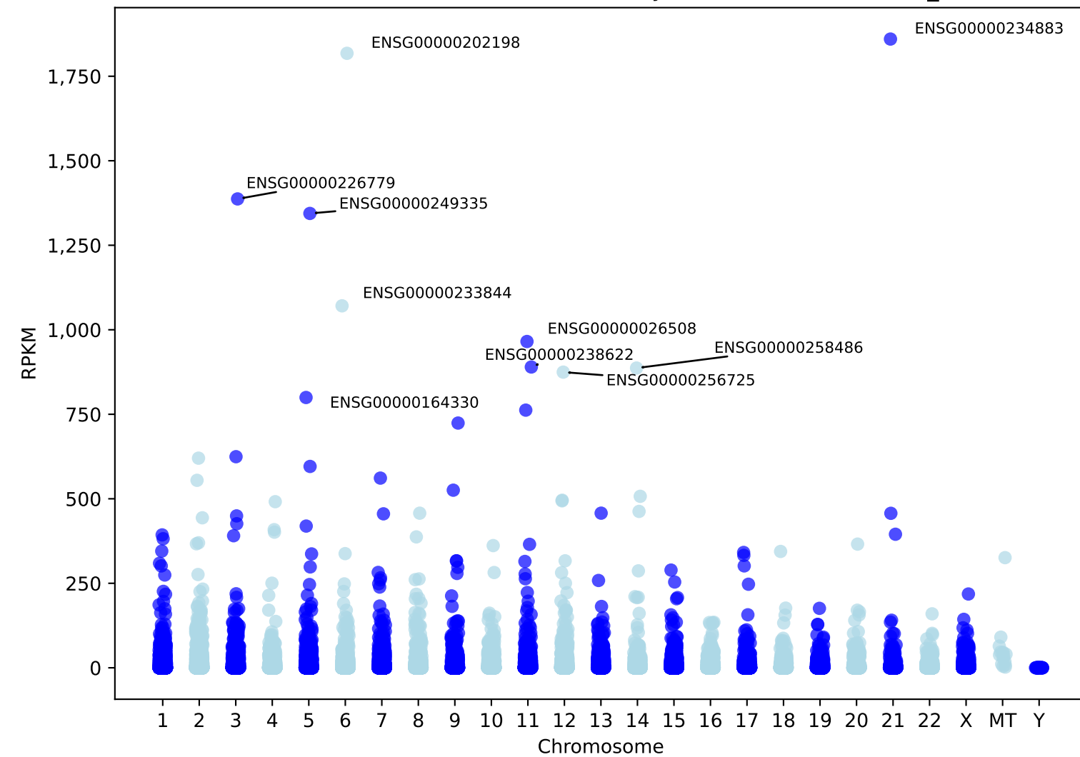
Scatter Plot of Total RPKM (all Reads) by Chromosome for ebna_hisat
