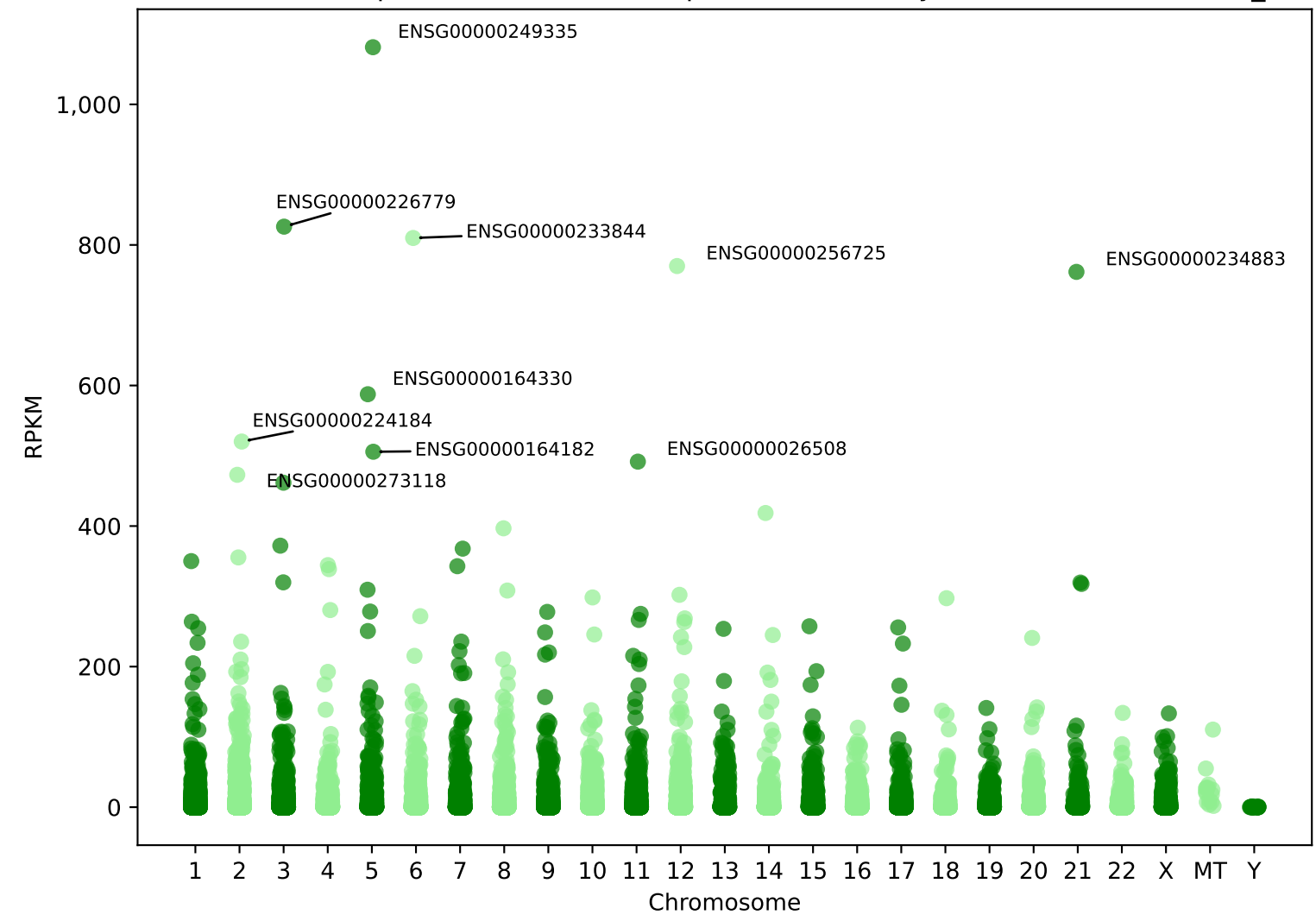
Scatter Plot of Unique RPKM (non-PCR duplicated reads) by Chromosome for ebna_hisat
