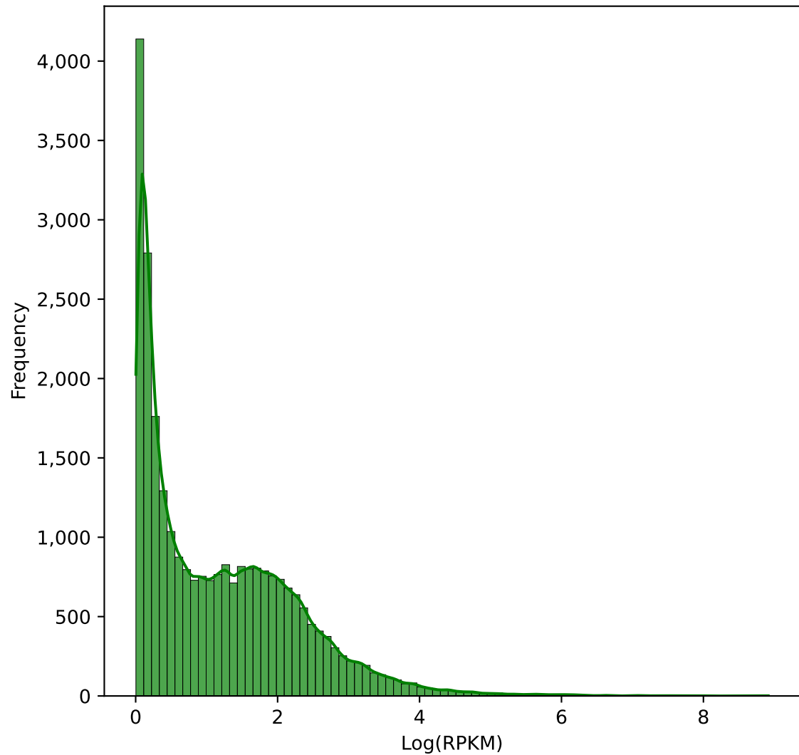
Log Distribution of Unique RPKM (non-PCR duplicated reads) for hes_star
