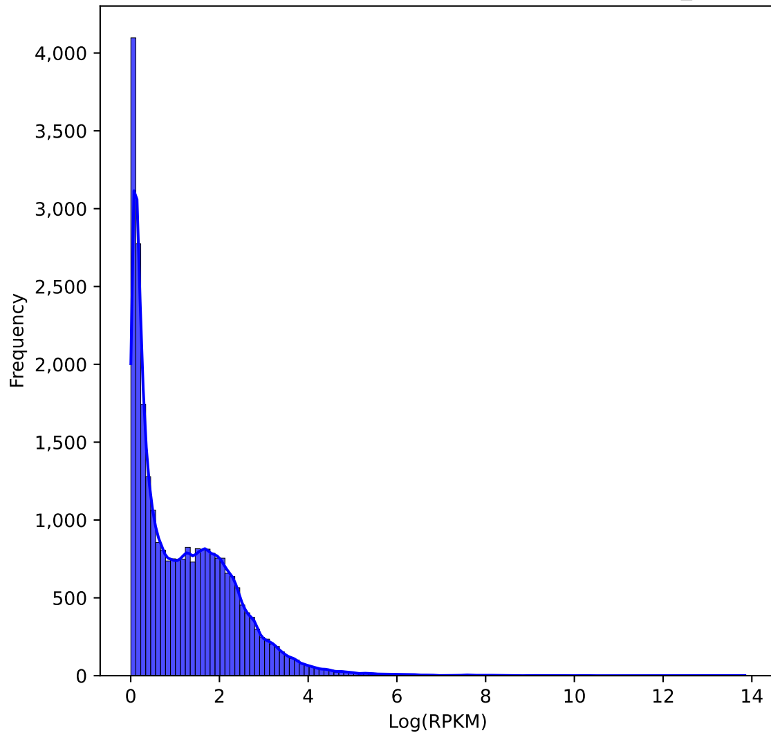
Log Distribution of Total RPKM (all Reads) for hes_star
