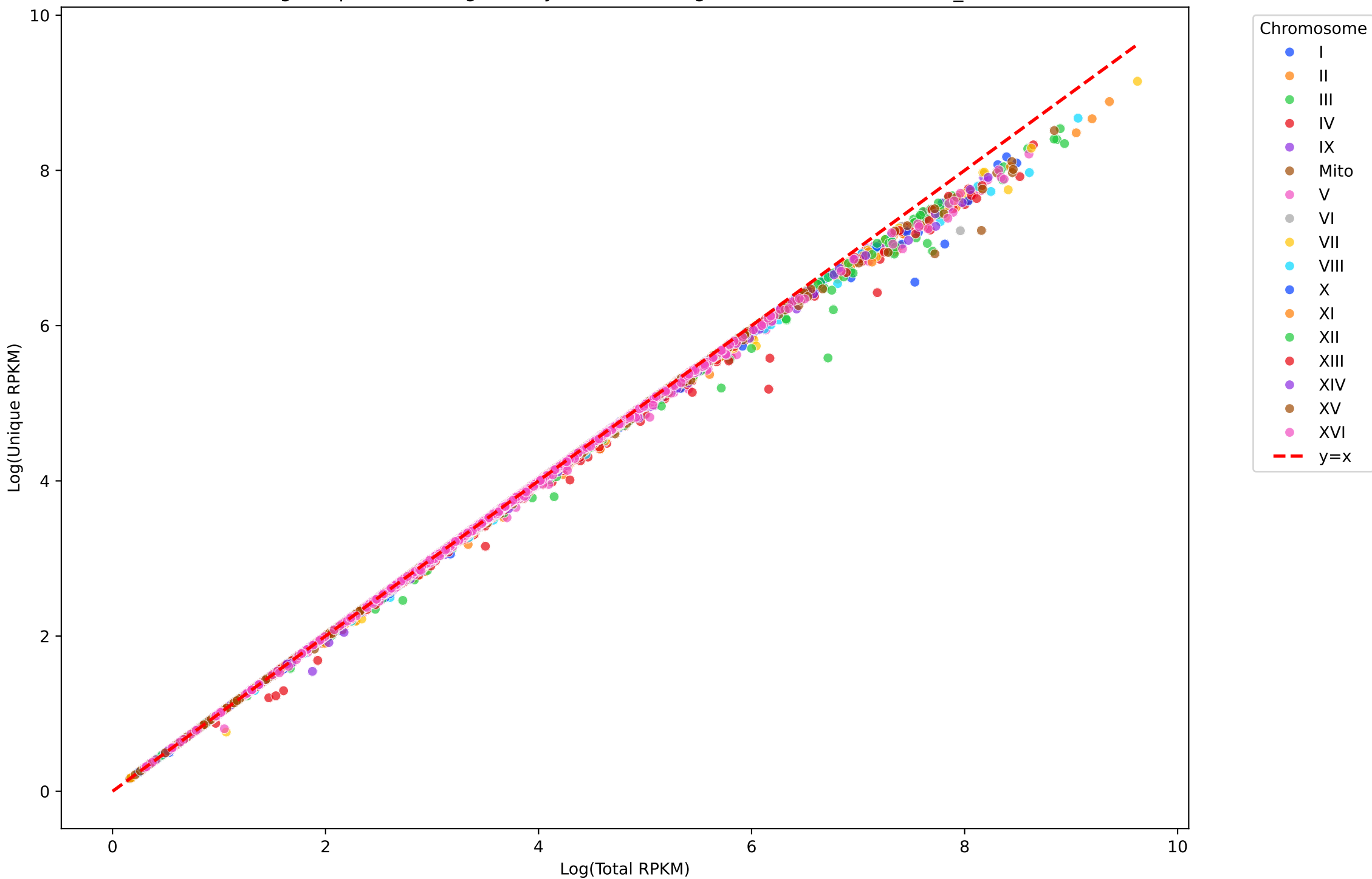
Log(Unique RPKM) is generally lower than Log(Total RPKM) for nookaew_cm
