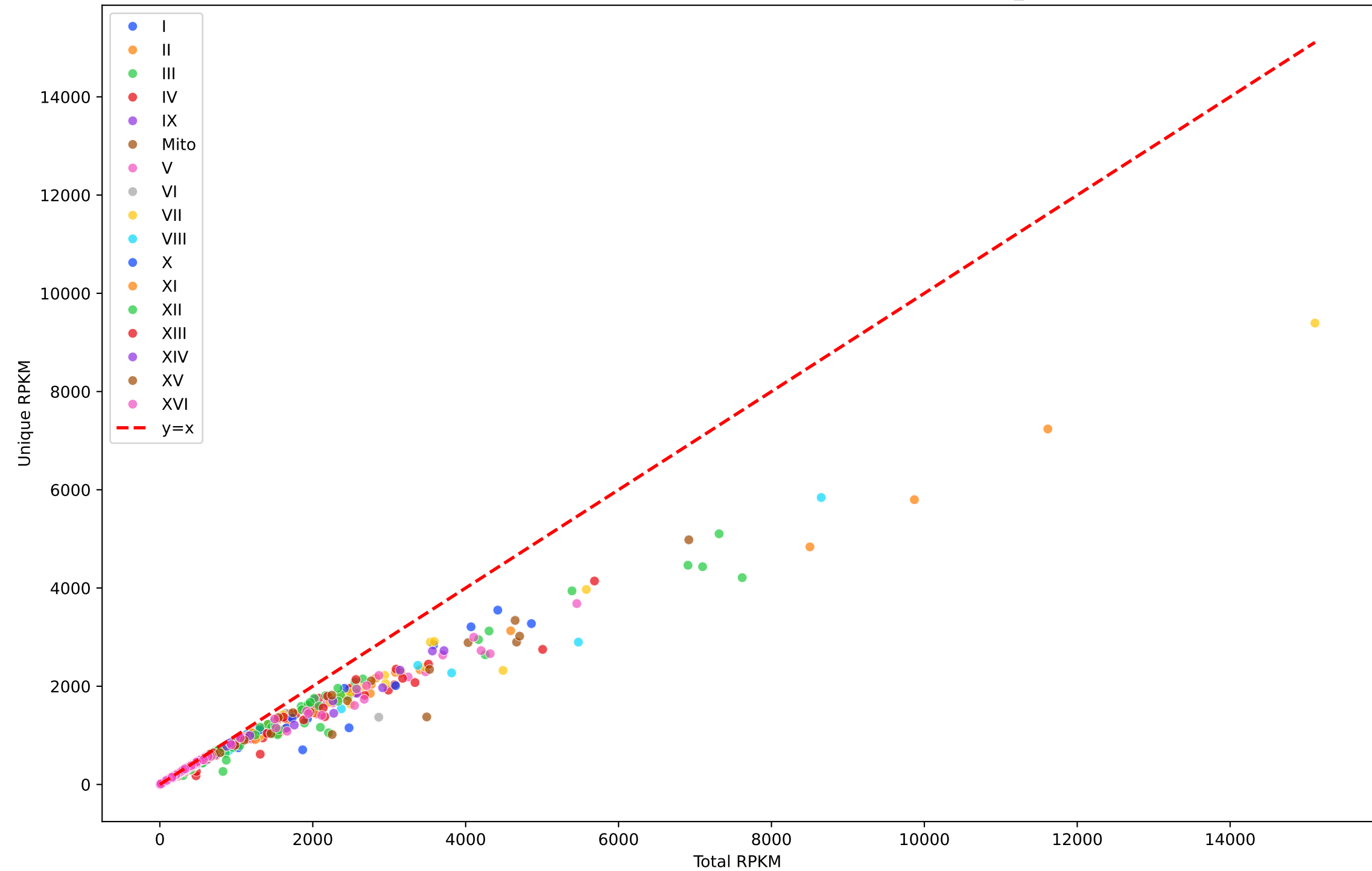
Unique RPKM is generally lower than Total RPKM for nookaew_cm
