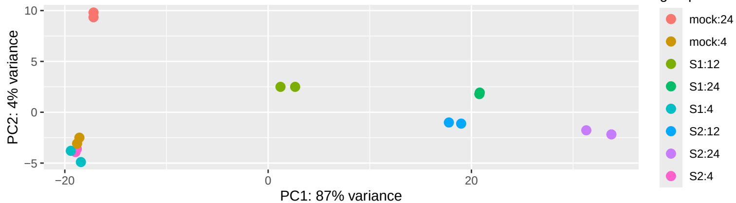
PCA Plot for star Analysis
