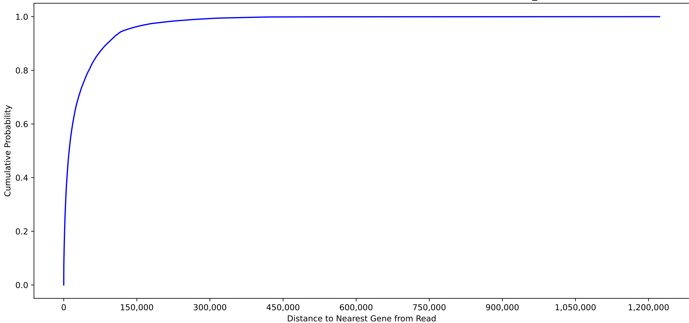
Cumulative Distribution Function of Distances to the Nearest Gene for ebna_hisat
