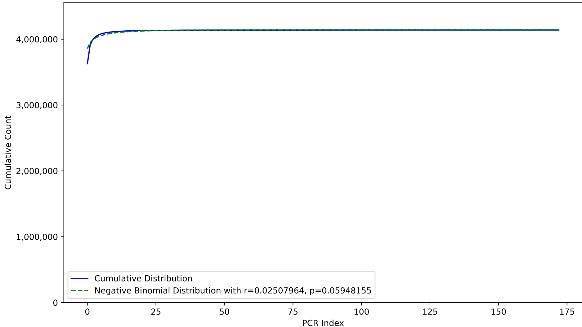
Cumulative Distribution of PCR Index Counts with Negative Binomial Fit for nookaew_cm
