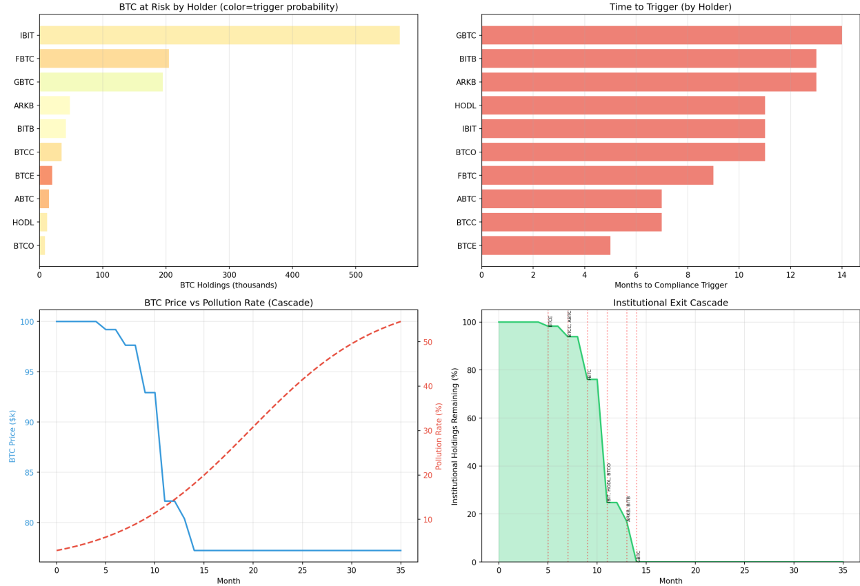
Figure 7: Figure 4: Institutional exit cascade simulation with Almgren-Chriss market impact. The figure presents four panels: (top-left) a horizontal bar chart of BTC holdings by ETF issuer color-coded by compliance trigger probability, with IBIT (~570K BTC) holding the largest position at lower trigger risk while smaller funds like BTCE face higher trigger probabilities; (top-right) estimated months to compliance trigger for each holder, ranging from approximately 4 to 14 months; (bottom-left) the simulated cascade timeline showing cumulative BTC sold and the resulting price trajectory under the Almgren-Chriss temporary and permanent impact decomposition; (bottom-right) sensitivity of total market impact to liquidation horizon, illustrating the classic execution-speed tradeoff where faster exits (10 days) produce ~3.5% impact versus ~2.3% for slower exits (90 days). The results demonstrate that orderly liquidation substantially mitigates cascade risk compared to naive forced-selling assumptions.
