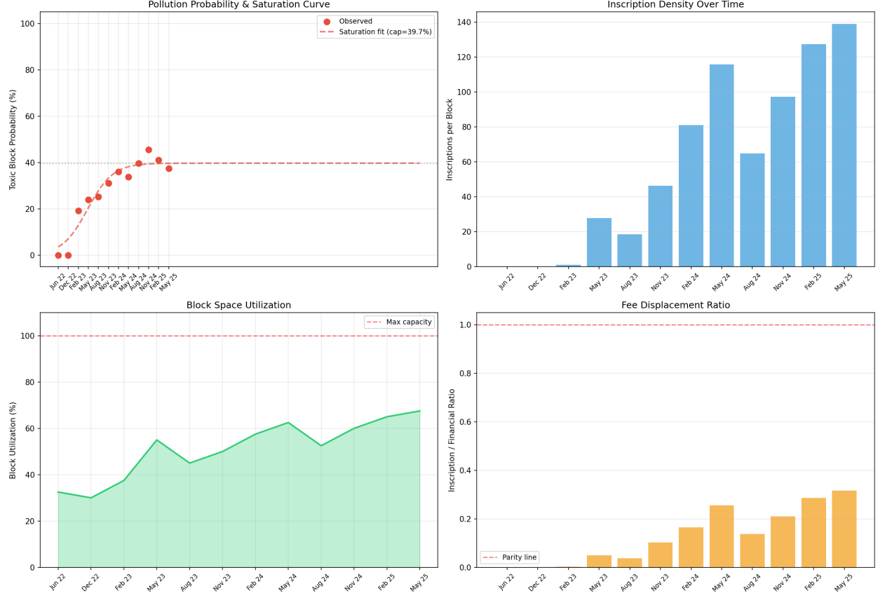
Figure 5: Figure 2: Content pollution probability and saturation curve with fee-market dampening. The figure comprises four subplots: (top-left) observed toxic block probability over time with a logistic saturation fit converging to a 39.7% asymptote, showing rapid growth after late 2022 that plateaus by mid-2023; (top-right) inscription density per block over time, with bars rising from near-zero pre-2023 to peaks exceeding 100 inscriptions per block; (bottom-left) the fee-market pushback multiplier as a function of average fee rate, illustrating how the dampening factor approaches zero at high fee levels and thereby suppresses low-value inscriptions; (bottom-right) the composite pollution score decomposed by weighted factor contributions. The saturation well below 100% confirms that the fee-auction mechanism provides an endogenous ceiling on content pollution, as modeled in Section 3.2.2.
