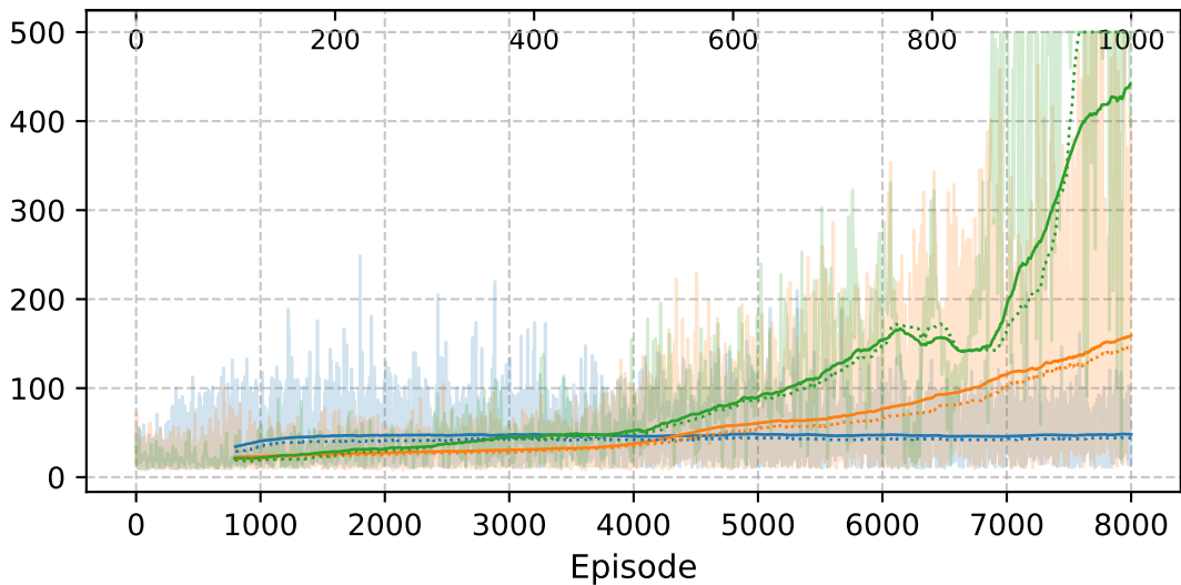
Total reward
