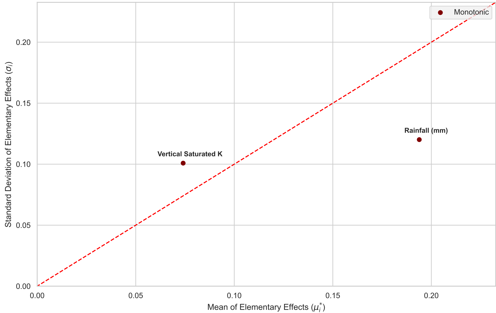
Morris sensitivity analysis indexes
