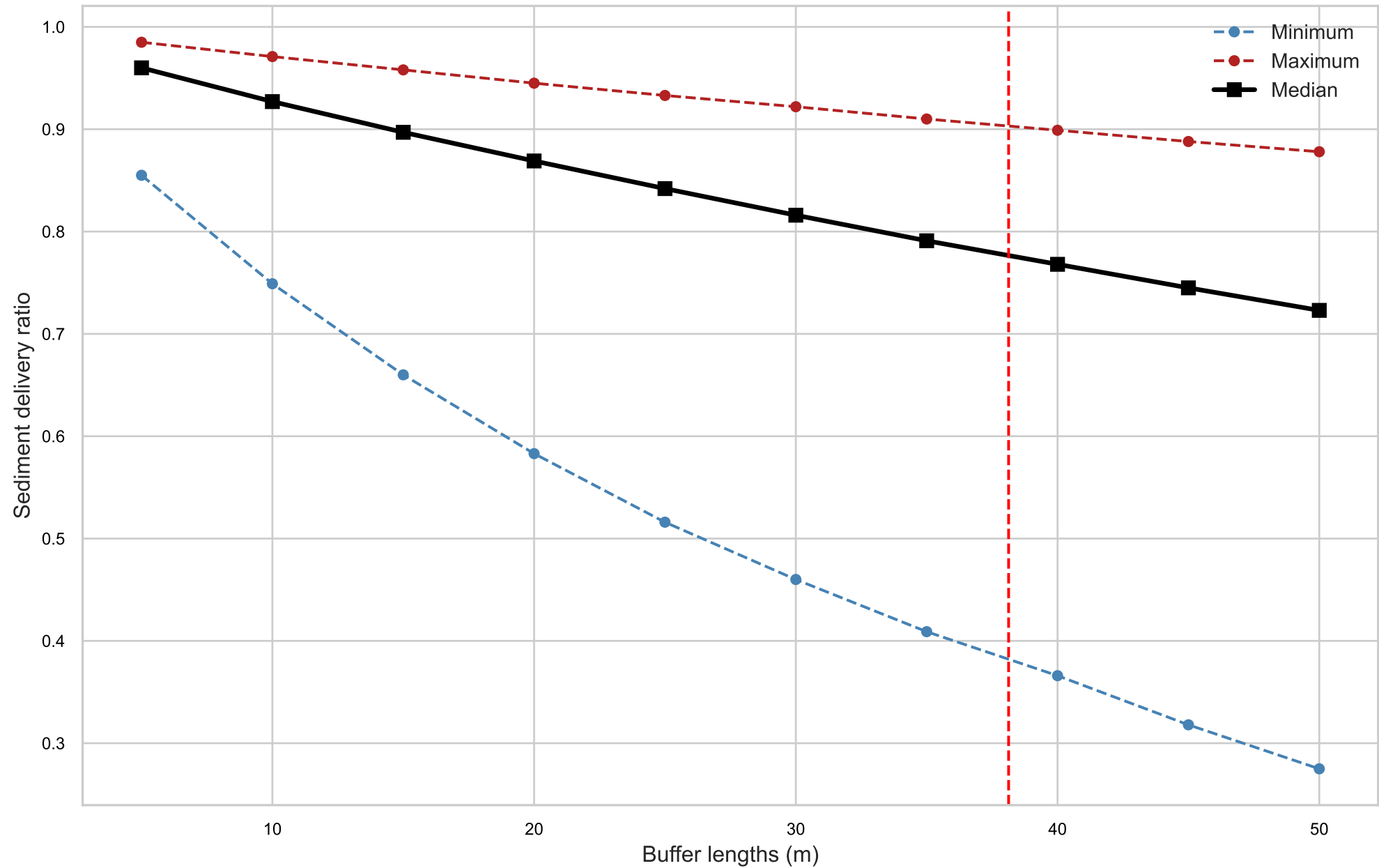
Buffer length for a sediment delivery ratio of 0.9
