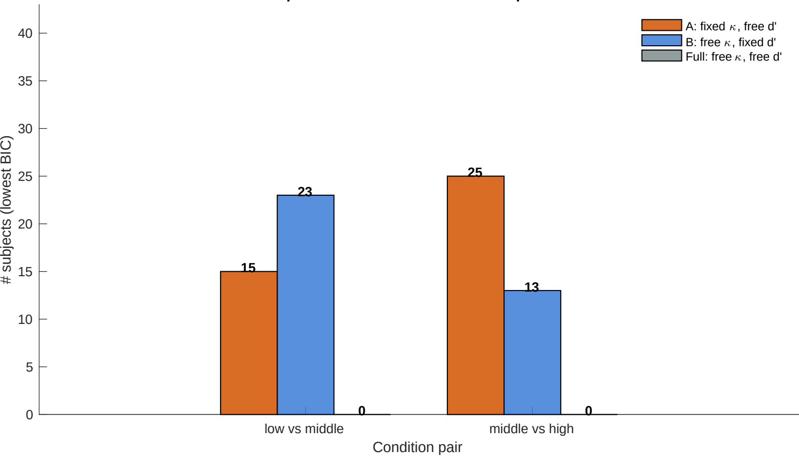
Exp 1 — TCC+vonMises model comparison
