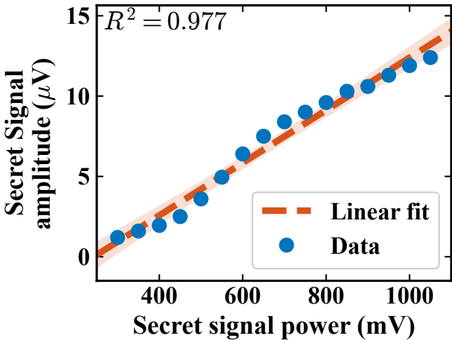
(a) Secret signal power vs. Secret signal amplitude
