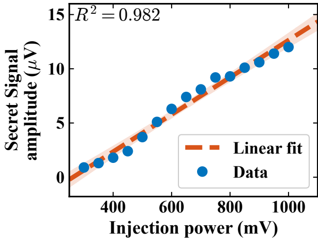
(b) Injection power vs. Secret signal amplitude
