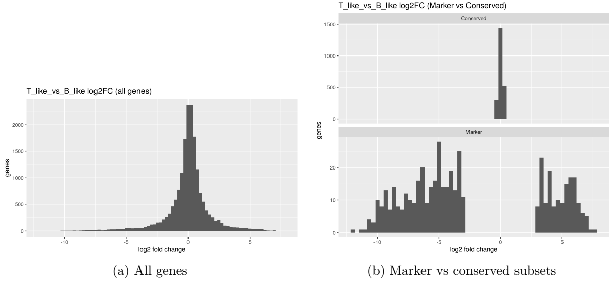
Figure 7: Distribution of DESeq2 log 2 fold-changes for a representative contrast (T-like vs B-like). Most genes concentrate near 0, while strict marker calls occupy the tails; equivalence calls concentrate near 0 by construction.
