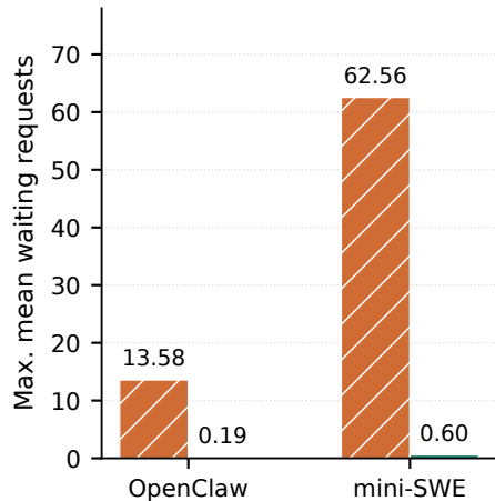
(c) Worst backend queue
