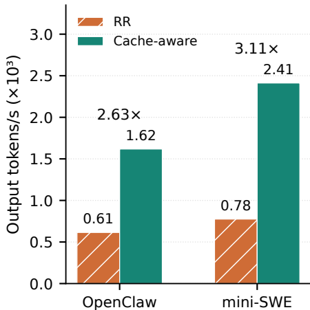
(a) Throughput gain
