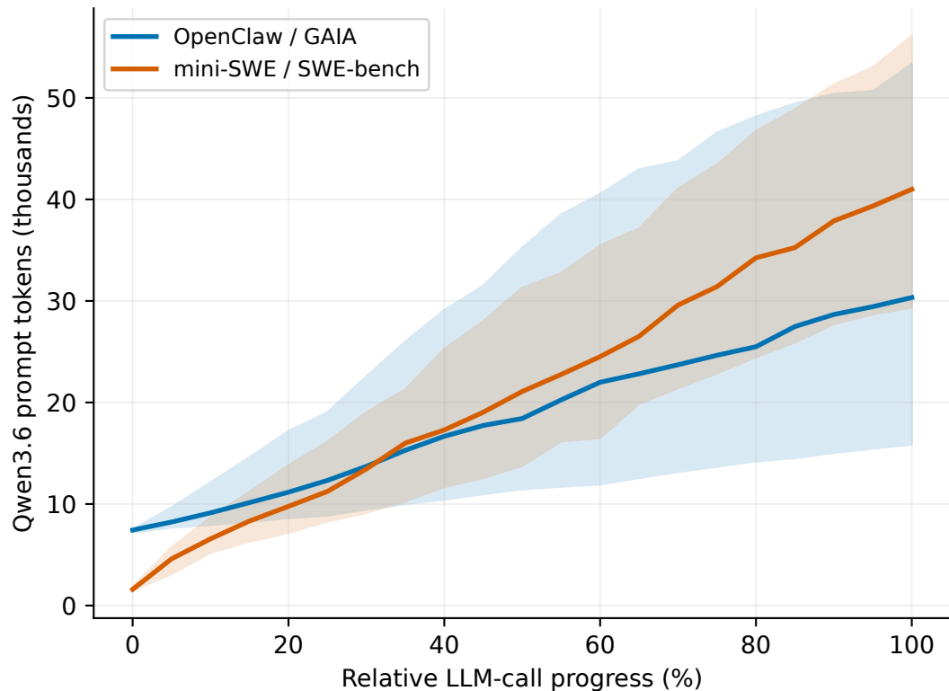
(a) Context growth: median and IQR
