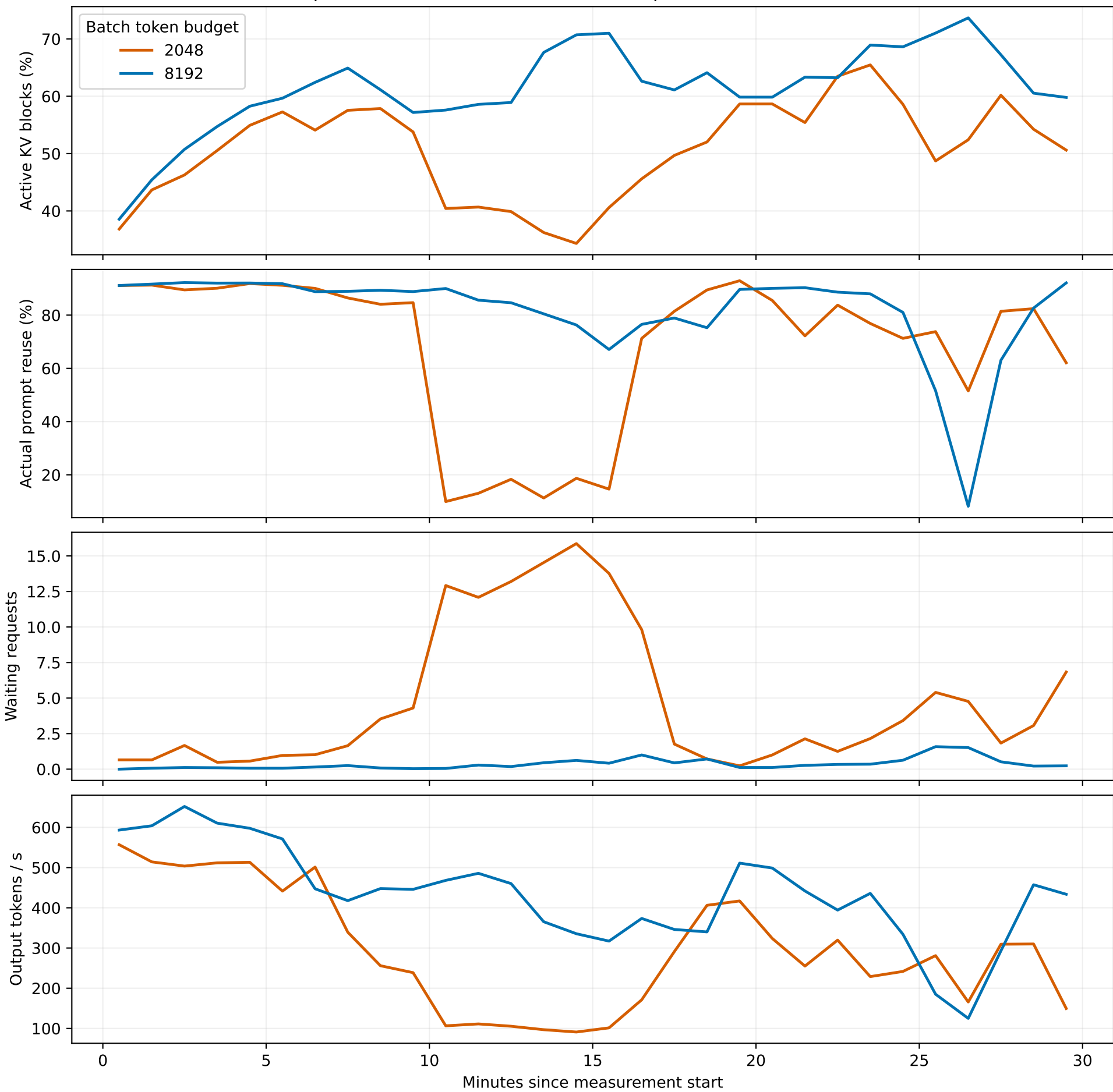
OpenClaw cc32: 2048 vs 8192 (same pool and seed, 60 s bins)
