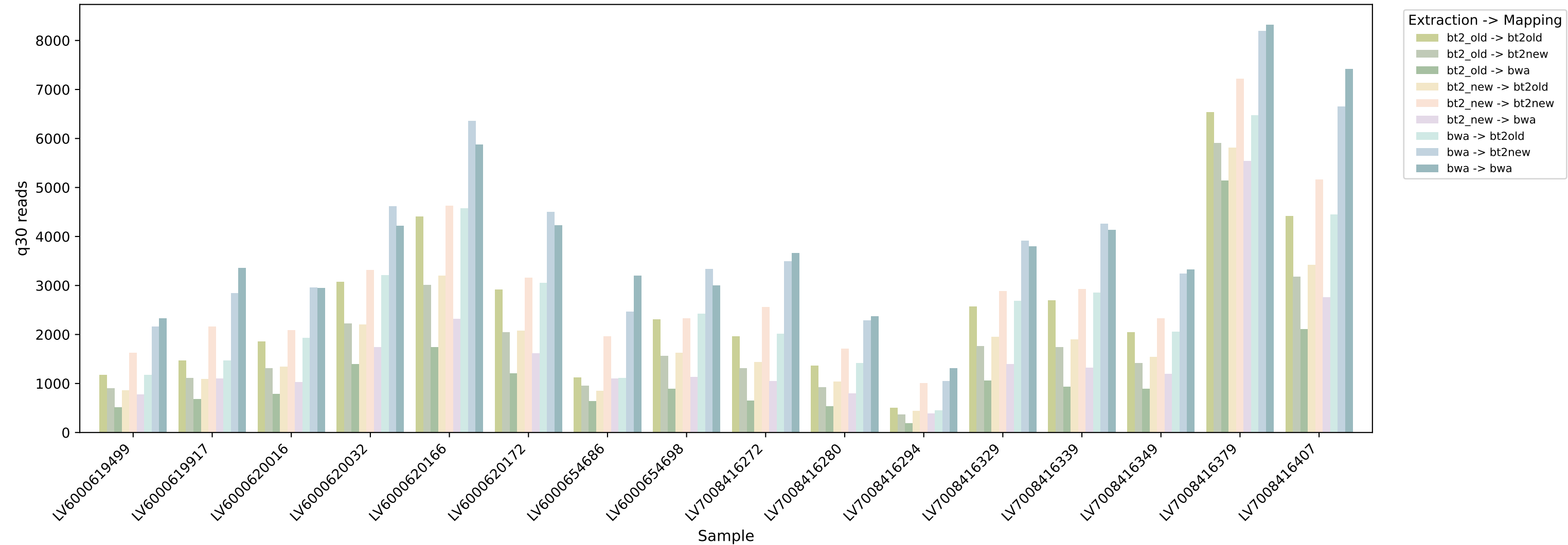
q30 Reads by Sample and Combo (16 samples x 9 combos)
