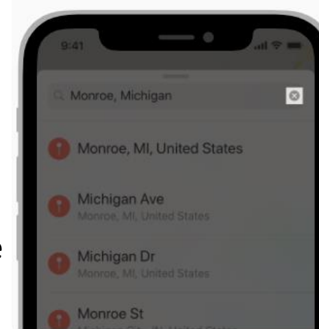
Clear button
