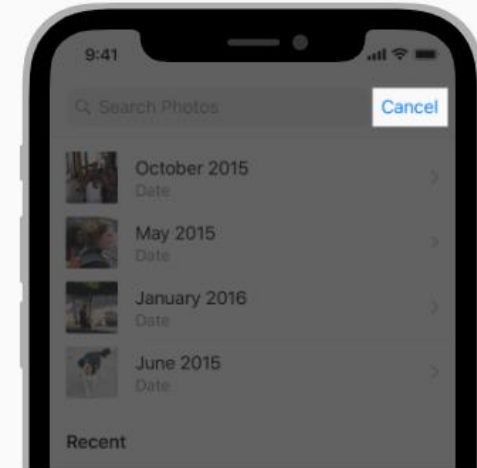
Cancel button
