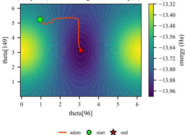
BeH2 (14 qubits) - sea convergence landscape (contour)
