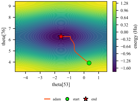
H4 (8 qubits) - local_global convergence landscape (contour)
