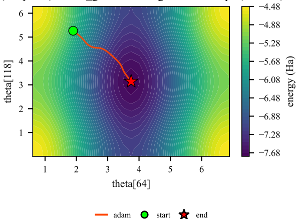
LiH (12 qubits) - local_global convergence landscape (contour)
