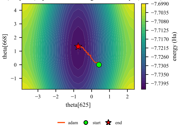
LiH (12 qubits) - pretrained convergence landscape (contour)
