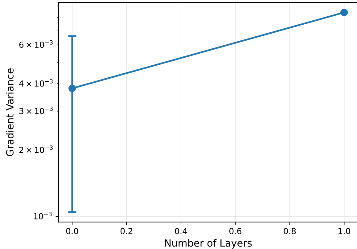
Variance vs Circuit Depth
