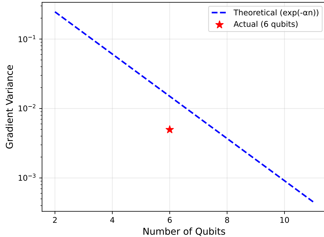
Variance Scaling with System Size
