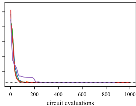
ADAM
