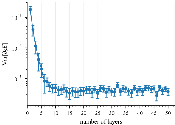
LiH (12 qubits): gradient-variance scaling
