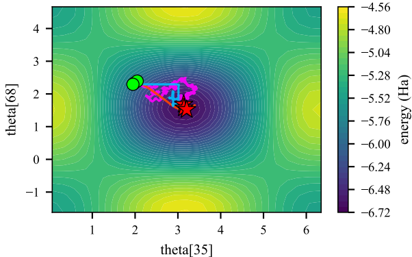
LiH (12 qubits) - local_global convergence landscape (contour)
