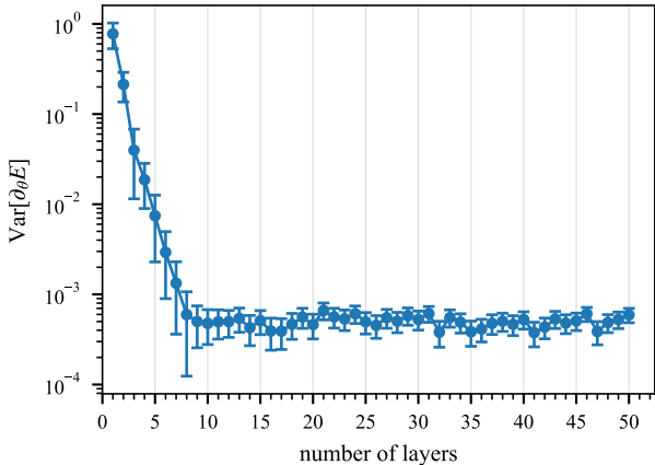
BeH2 (14 qubits): gradient-variance scaling
