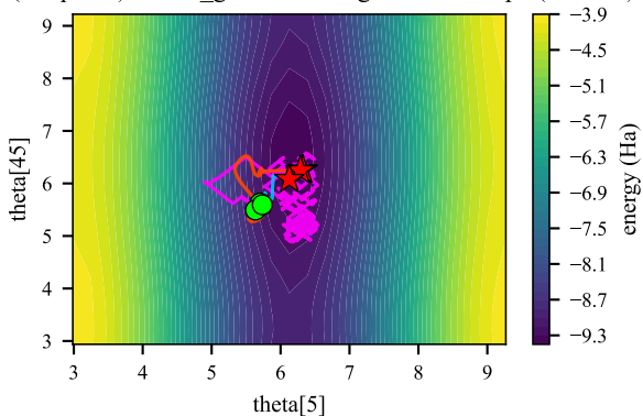
BeH2 (14 qubits) - local_global convergence landscape (contour)
