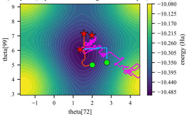
BeH2 (14 qubits) - pretrained convergence landscape (contour)
