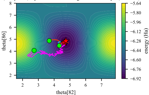
LiH (12 qubits) - pretrained convergence landscape (contour)
