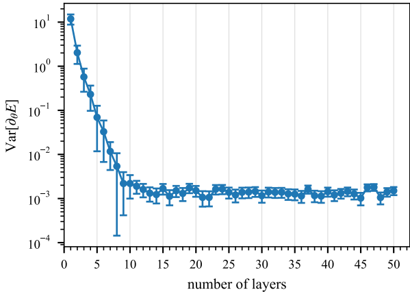
NH3 (16 qubits): gradient-variance scaling
