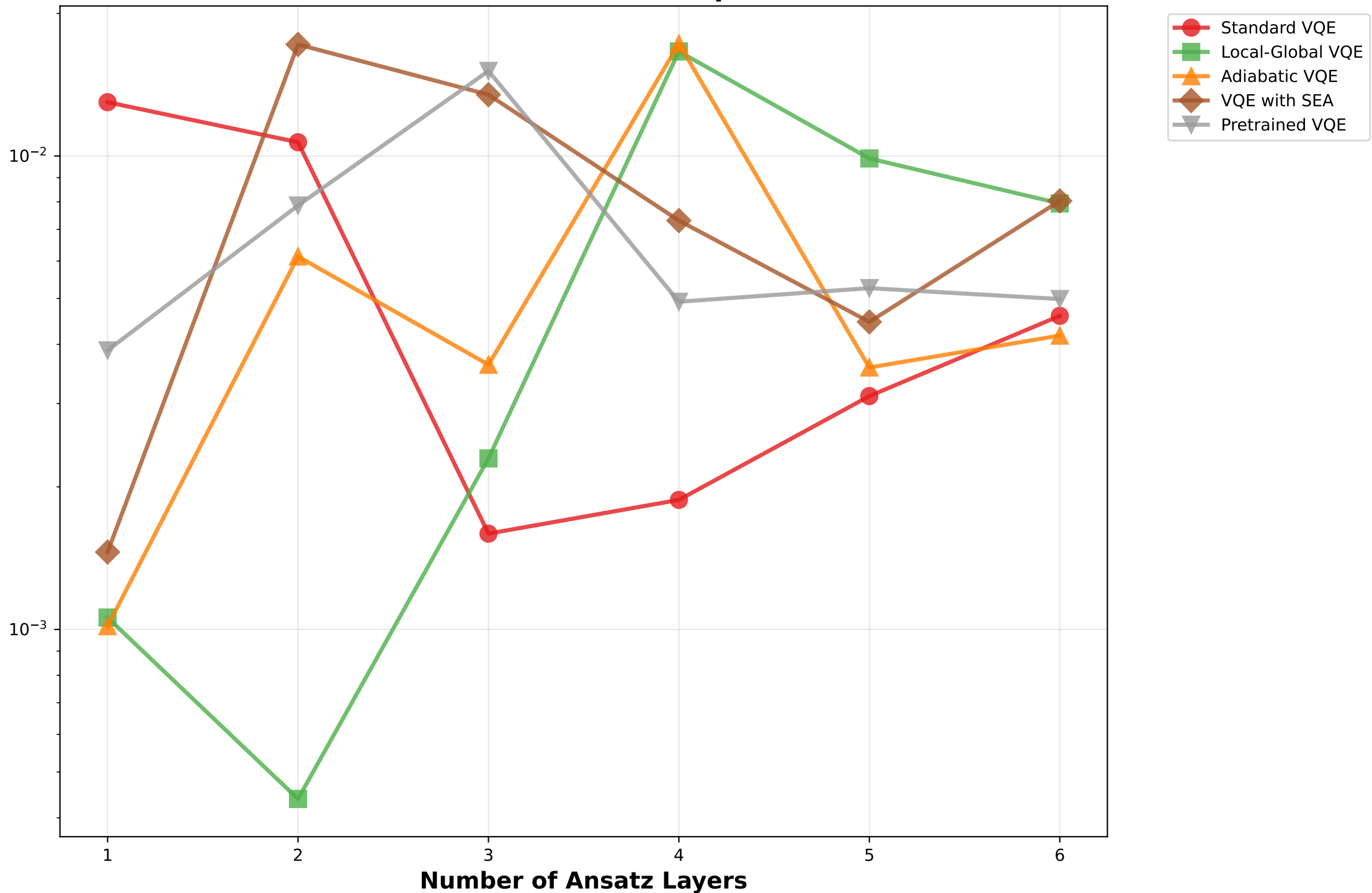
Gradient Variance vs Ansatz Depth (3 Qubits)
