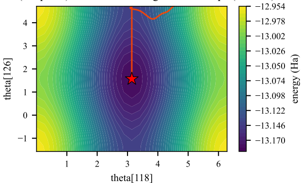
BeH2 (14 qubits) - standard convergence landscape (contour)
