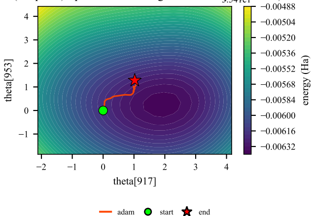
NH3 (16 qubits) - pretrained convergence landscape (contour)
